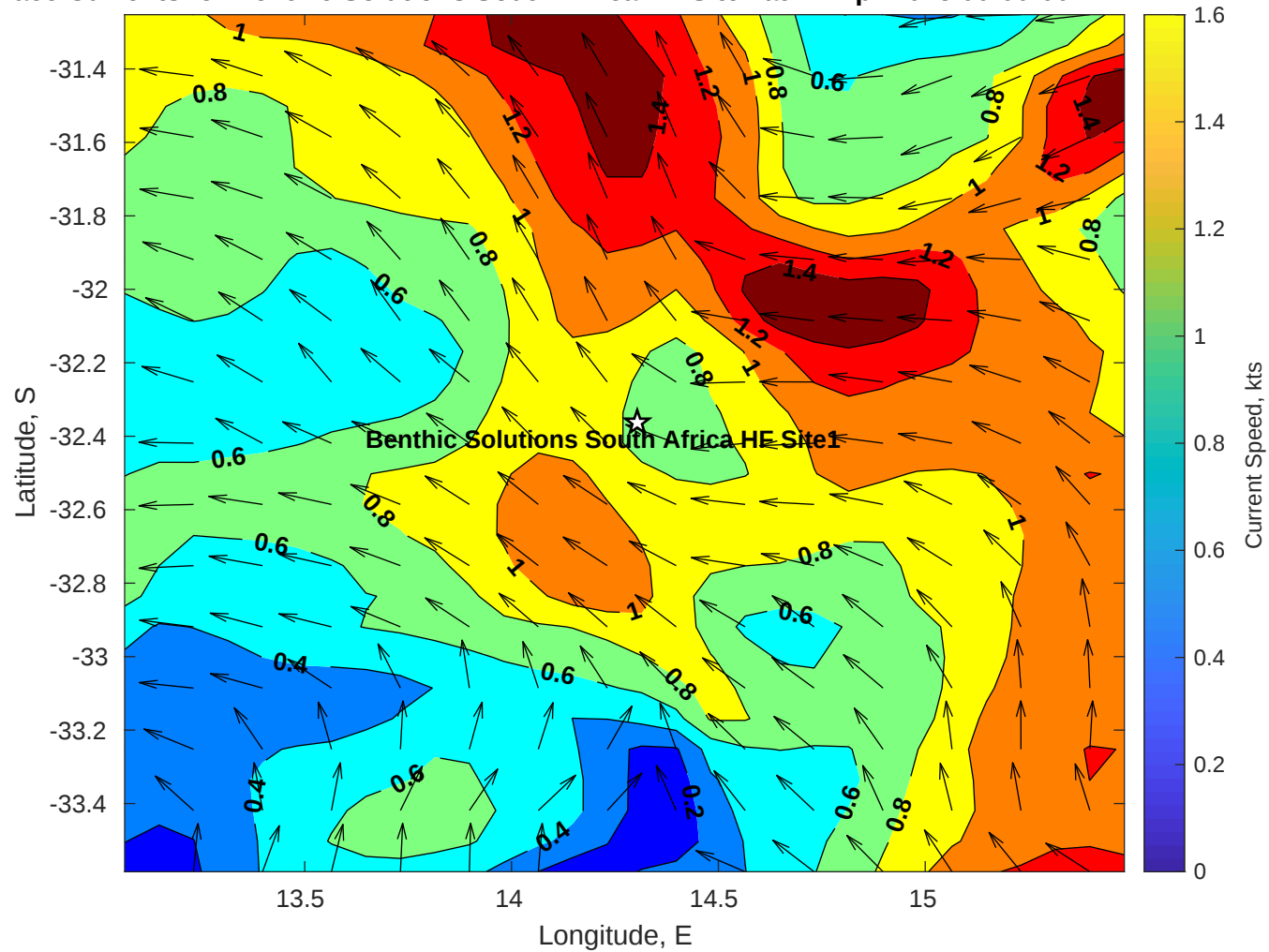
Surface Currents for Benthic Solutions South Africa HF Site1 at 21-Apr-2025 00:00:00
