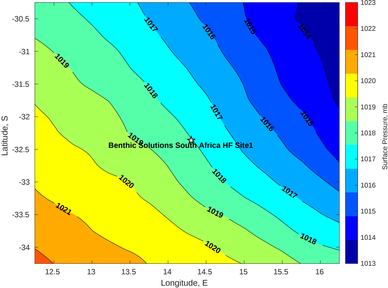
Surface Pressure (mb) for Benthic Solutions South Africa HF Site1 at 22-Apr-2025 00:00:00
