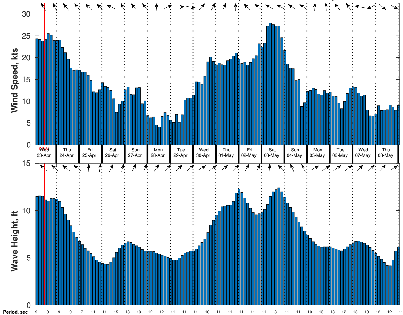
Wind & Wave Forecast for Benthic Solutions South Africa HF Site1 from 22-Apr-2025 02:00:00 to 08-May-2025 02:00:00
