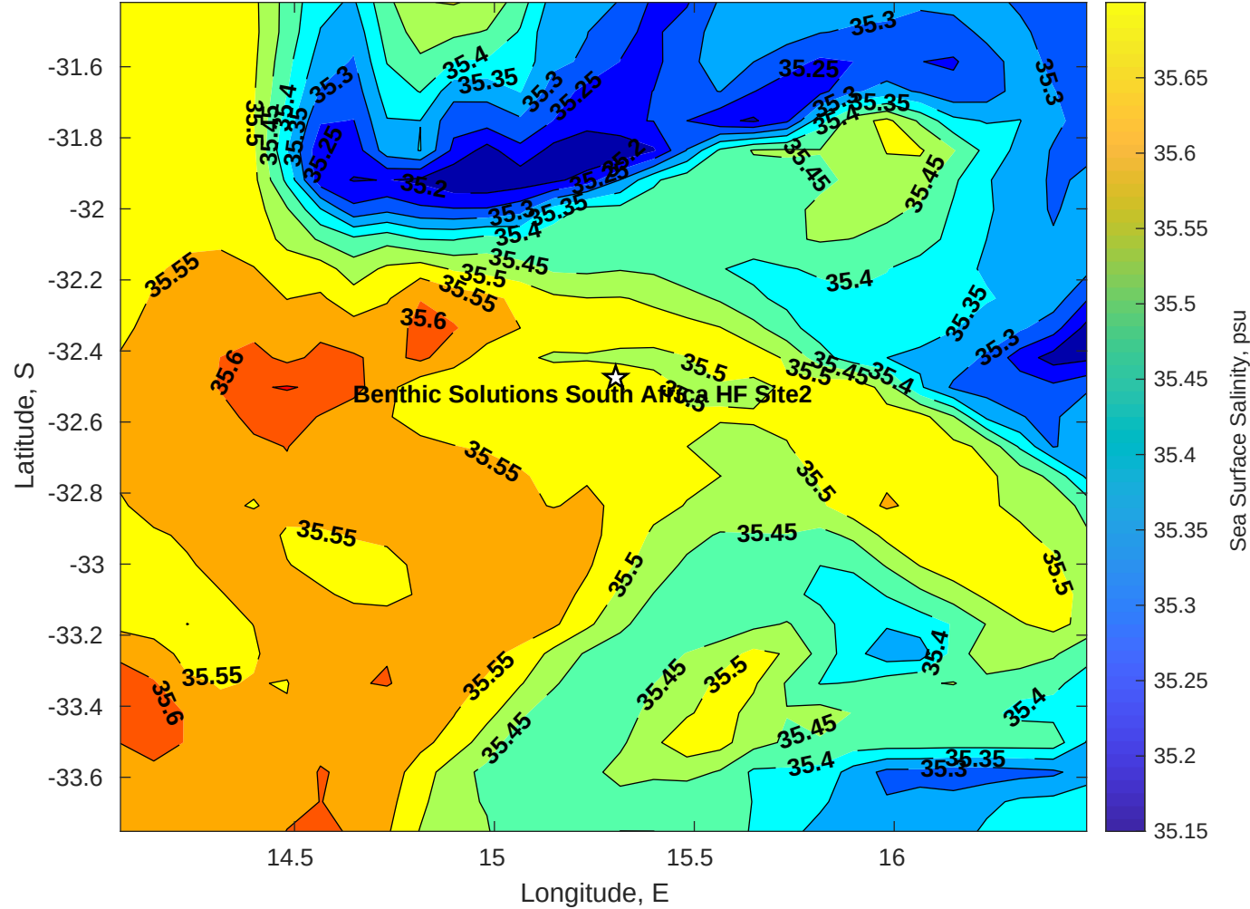
Surface Salinity for Benthic Solutions South Africa HF Site2 at 21-Apr-2025 00:00:00
