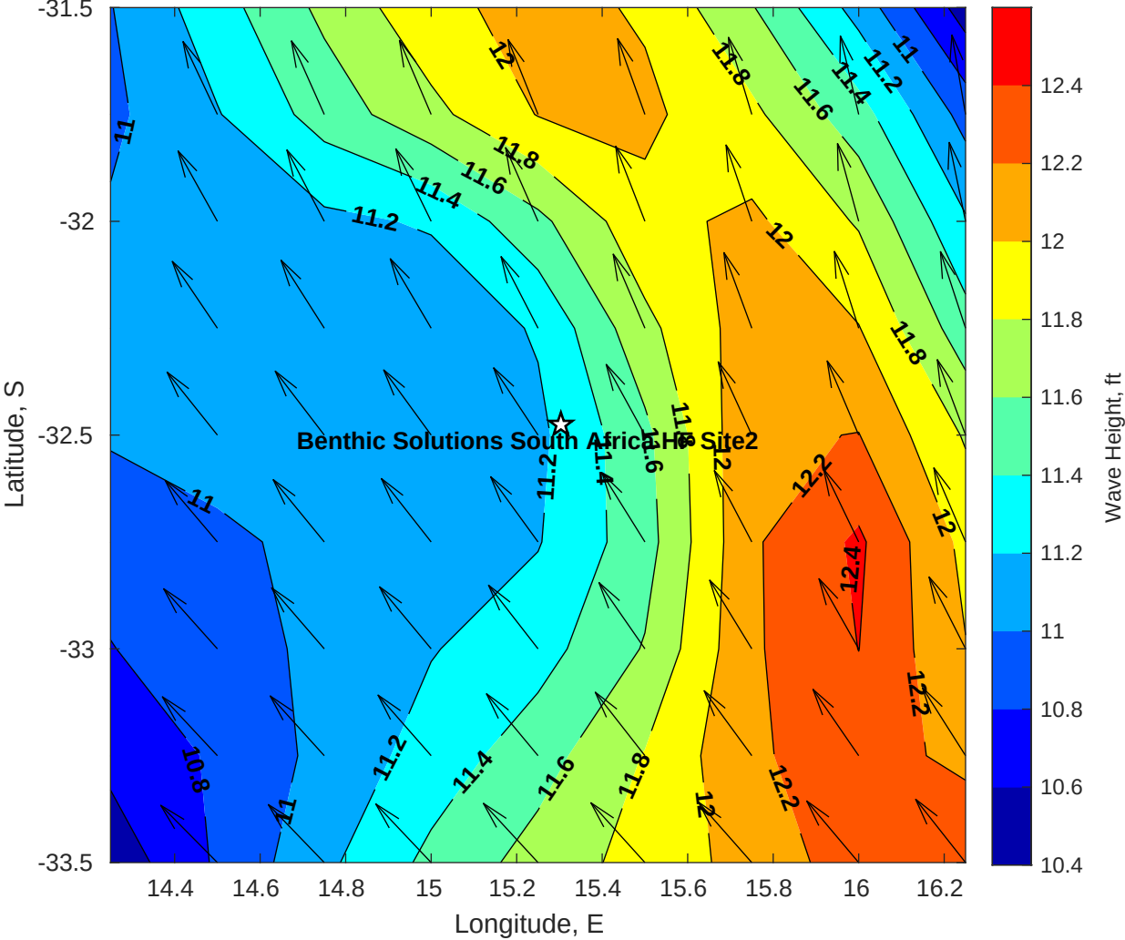
Wave Height (ft) for Benthic Solutions South Africa HF Site2 at 22-Apr-2025 09:00:00
