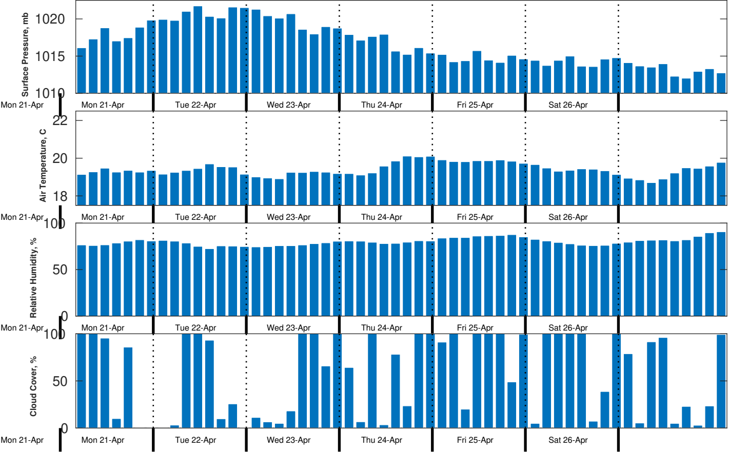
Met Forecast for Benthic Solutions South Africa HF Site2 from 22-Apr-2025 00:00:00 to 29-Apr-2025 00:00:00
