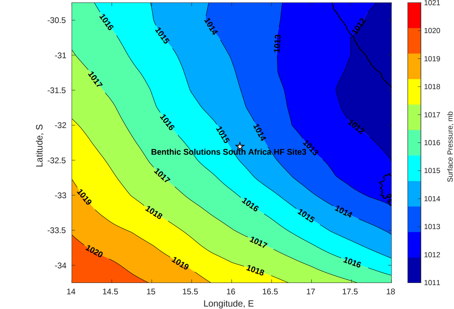
Surface Pressure (mb) for Benthic Solutions South Africa HF Site3 at 22-Apr-2025 00:00:00
