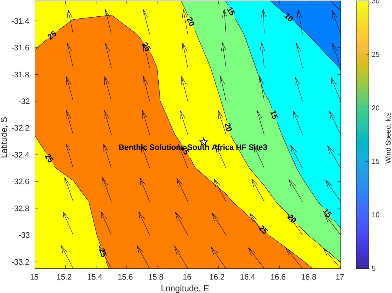
Winds (kts) for Benthic Solutions South Africa HF Site3 at 22-Apr-2025 09:00:00
