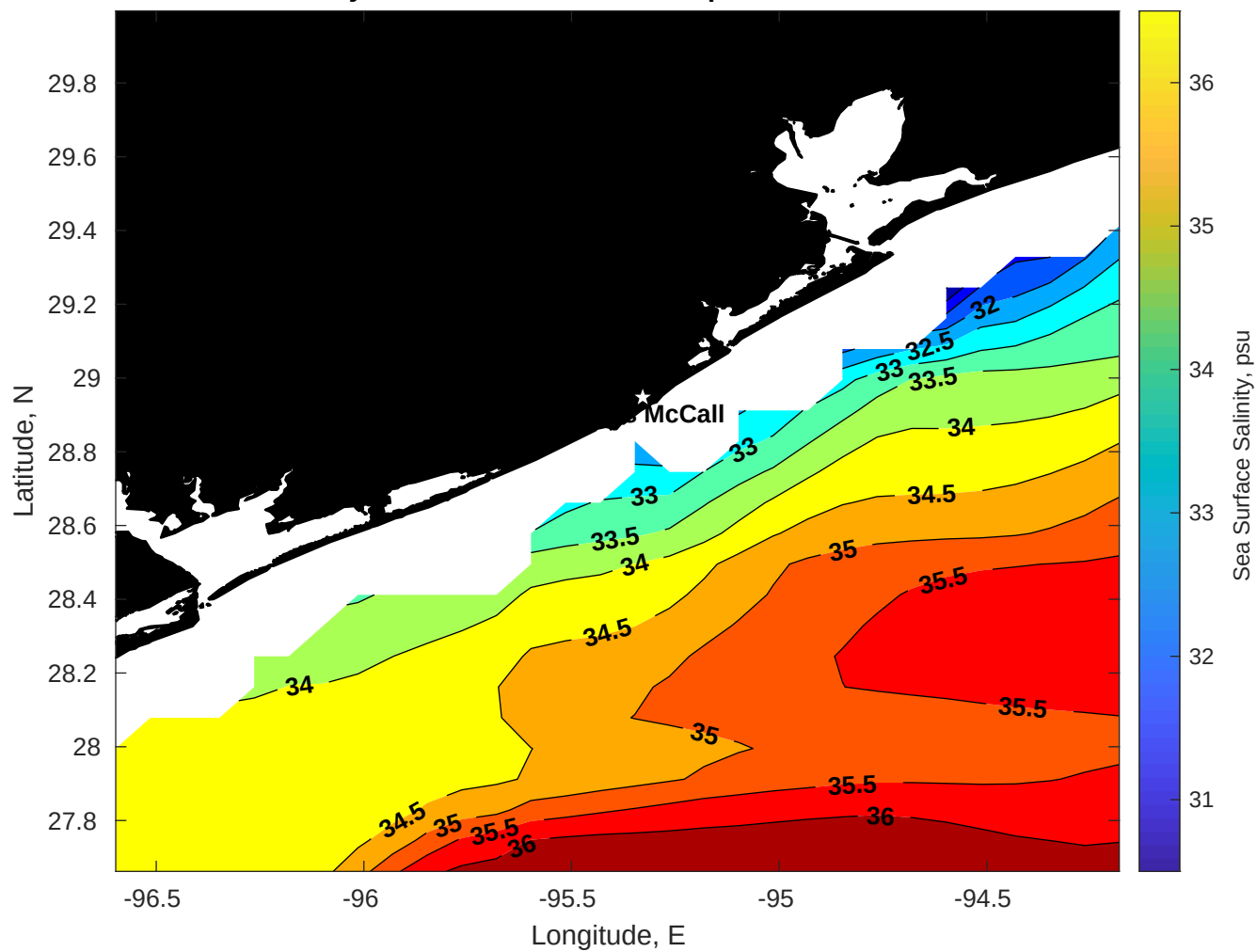
Surface Salinity for Brooks McCall at 21-Apr-2025 00:00:00
