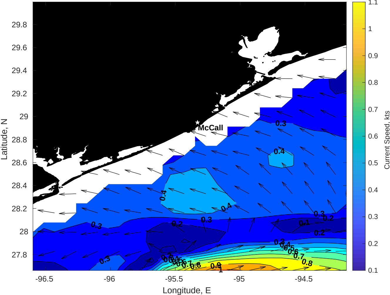
Surface Currents for Brooks McCall at 21-Apr-2025 00:00:00
