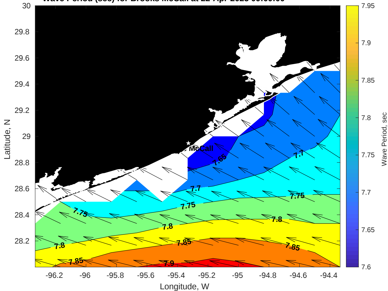
Wave Period (sec) for Brooks McCall at 22-Apr-2025 09:00:00
