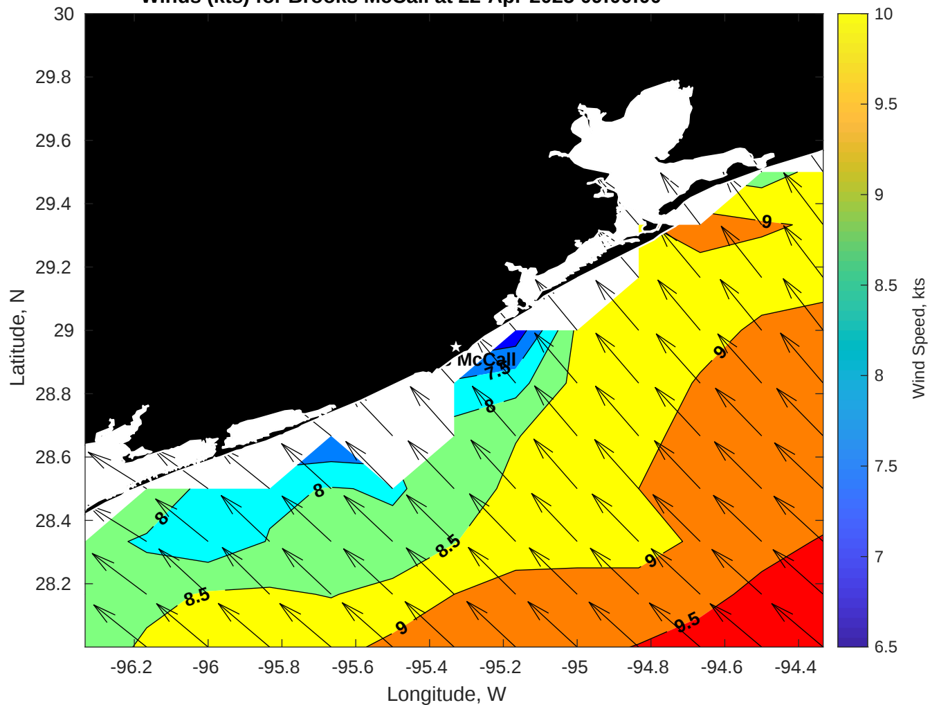
Winds (kts) for Brooks McCall at 22-Apr-2025 09:00:00
