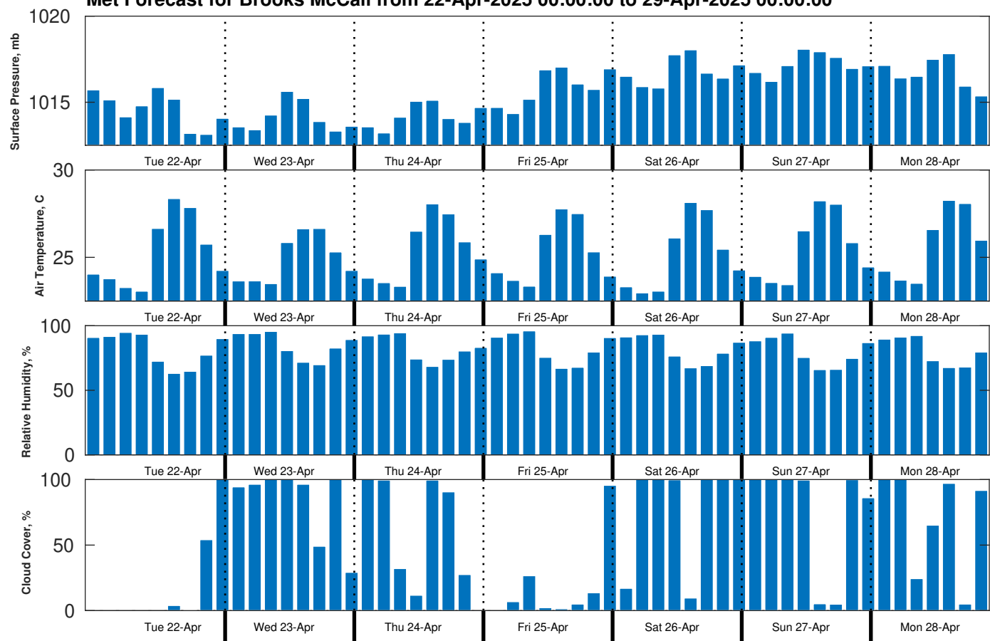
Met Forecast for Brooks McCall from 22-Apr-2025 00:00:00 to 29-Apr-2025 00:00:00
