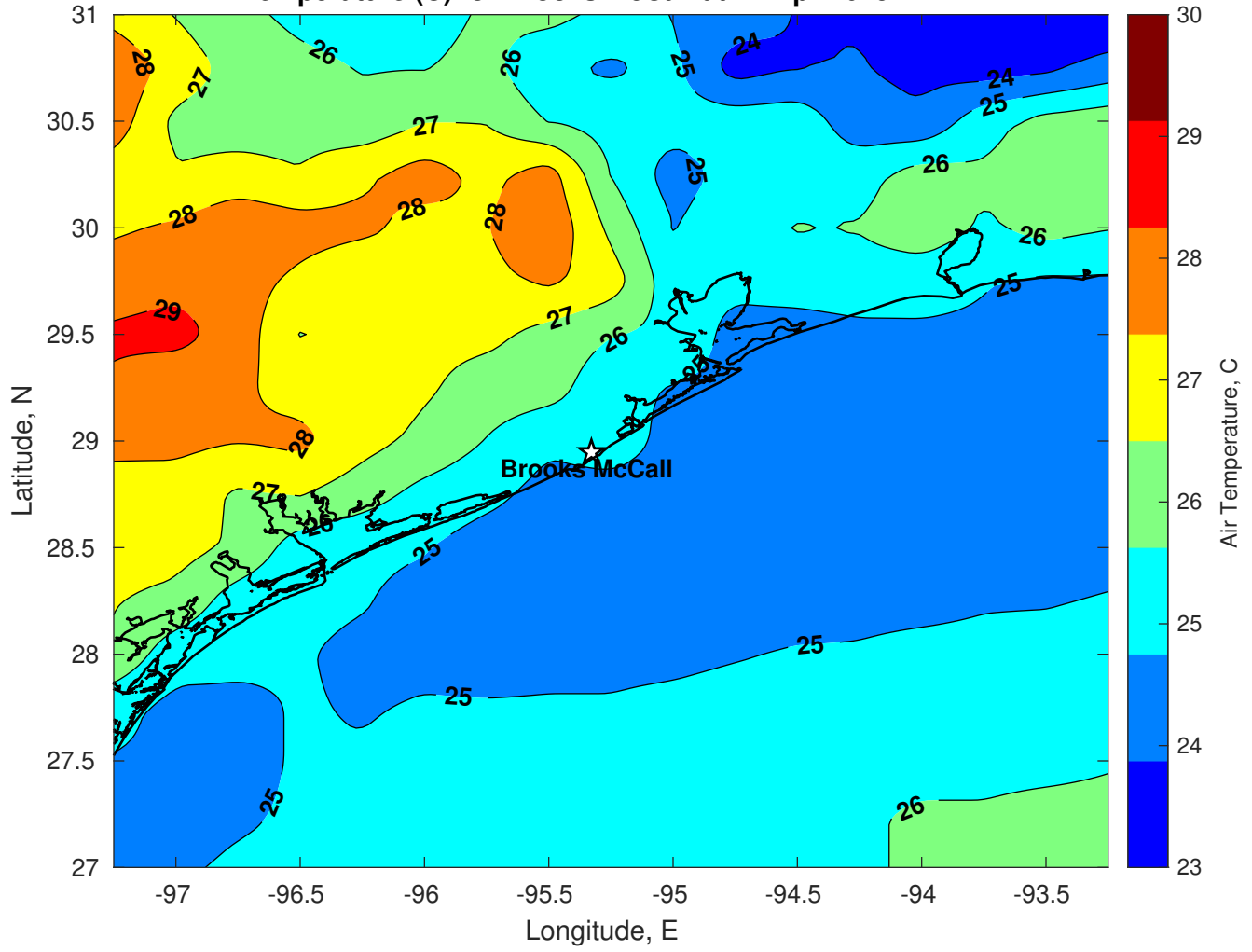
Air Temperature (C) for Brooks McCall at 22-Apr-2025
