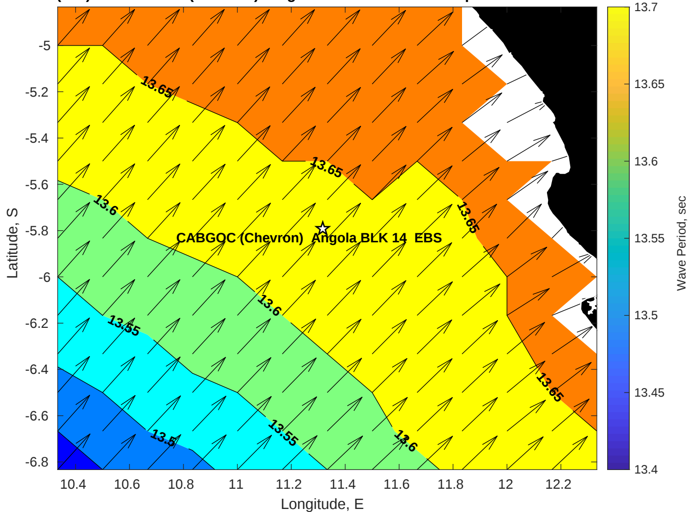
Wave Period (sec) for CABGOC (Chevron) Angola BLK 14 EBS at 22-Apr-2025 09:00:00
