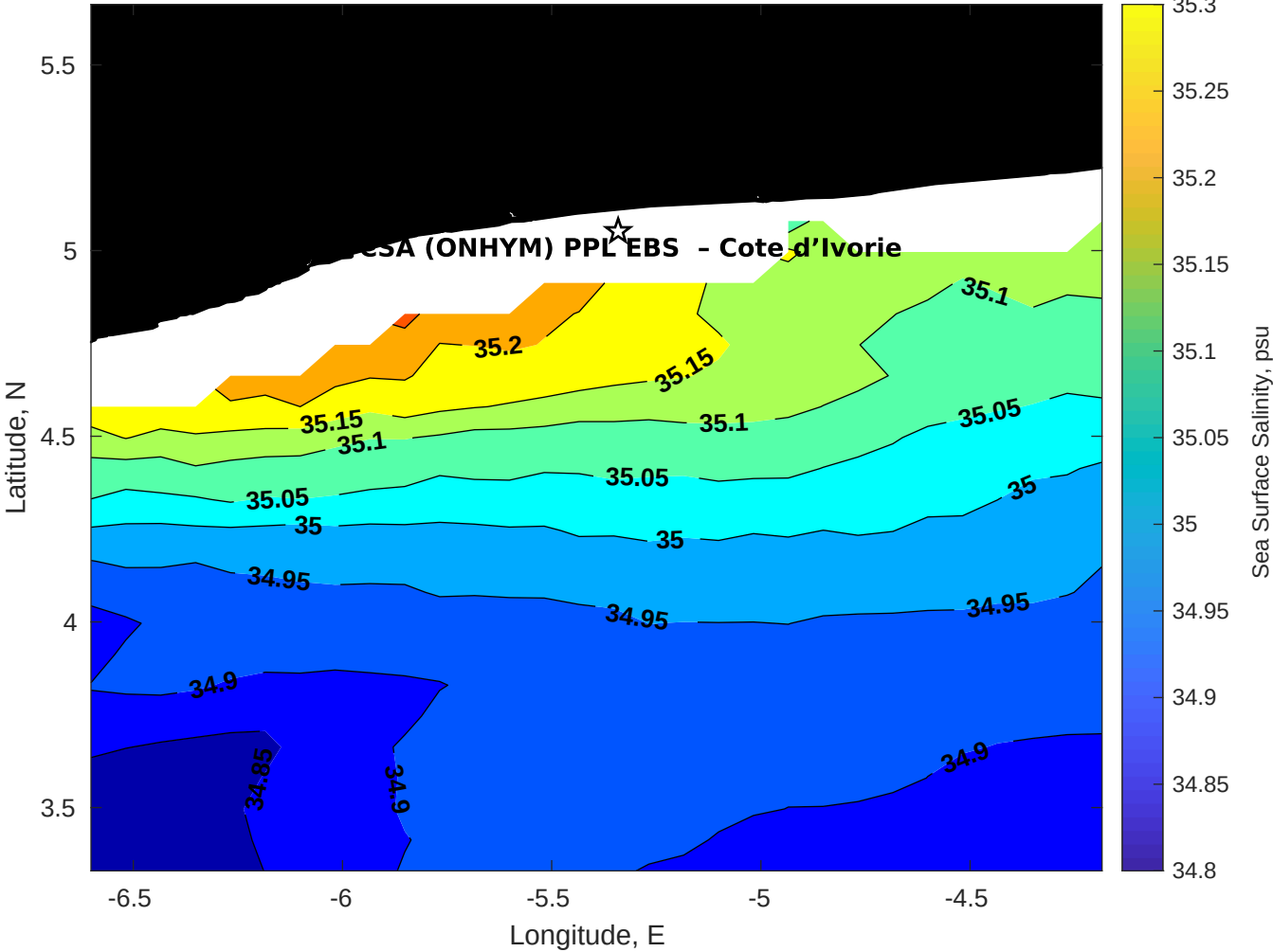
Surface Salinity for CSA (ONHYM) PPL EBS - Cote d'Ivoire at 21-Apr-2025 00:00:00
