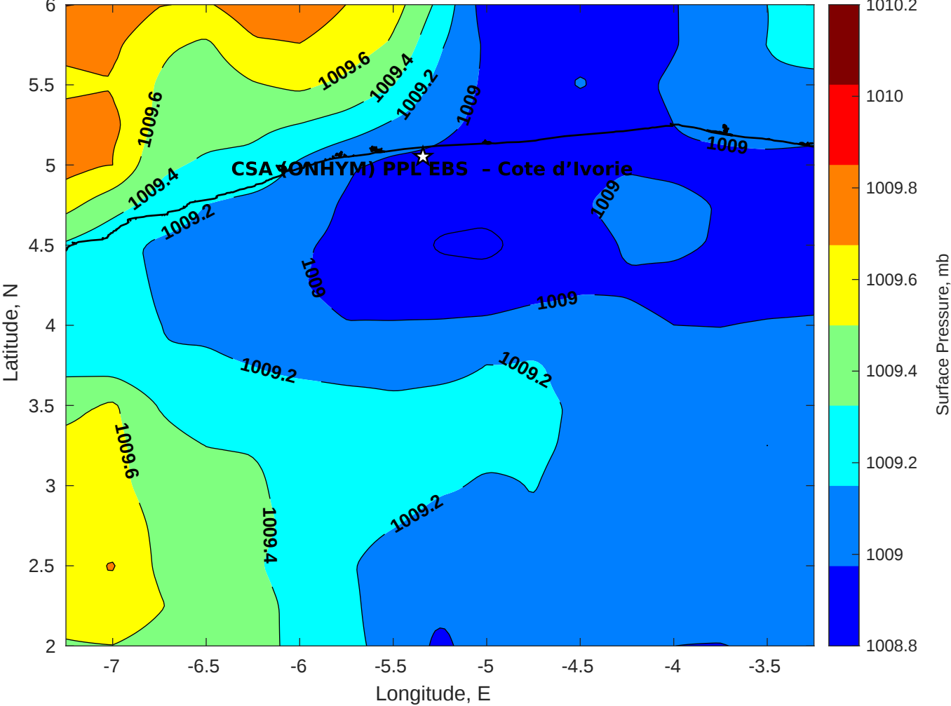
Surface Pressure (mb) for CSA (ONHYM) PPL EBS - Cote d'Ivoire at 22-Apr-2025 00:00:00
