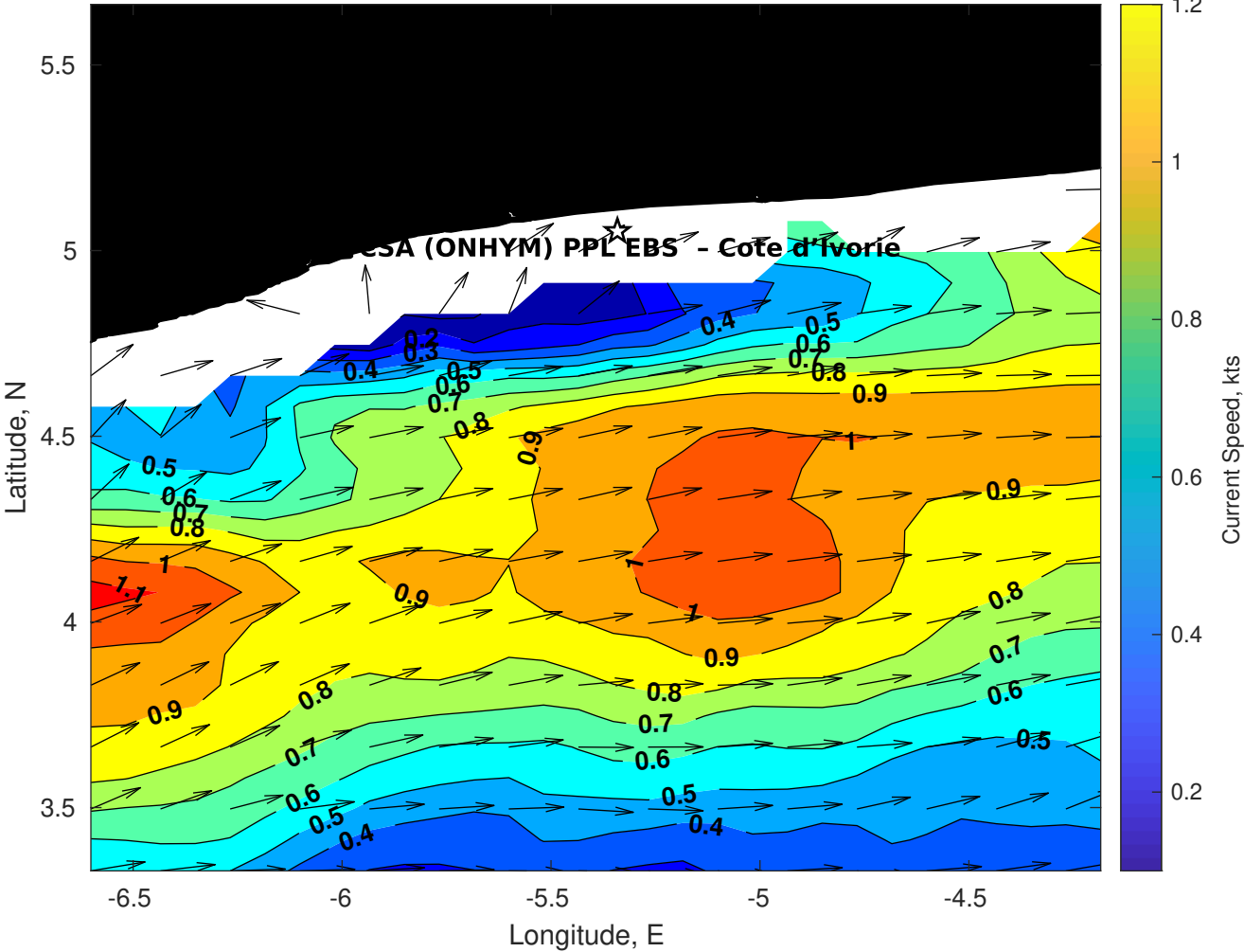
Surface Currents for CSA (ONHYM) PPL EBS - Cote d'Ivoire at 21-Apr-2025 00:00:00
