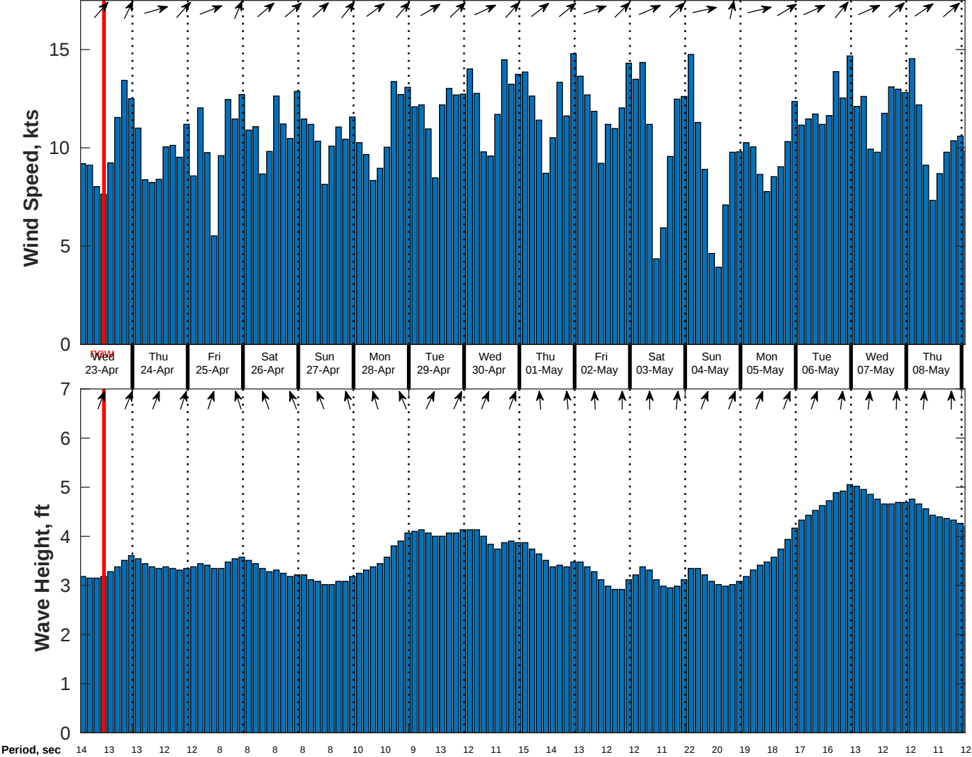
Wind & Wave Forecast for CSA (ONHYM) PPL EBS - Cote d'Ivoire from 22-Apr-2025 01:00:00 to 08-May-2025 01:00:00
