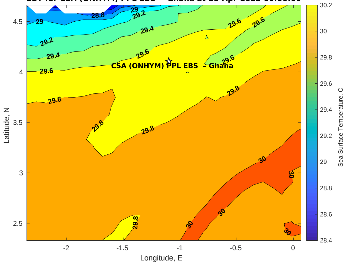
SST for CSA (ONHYM) PPL EBS - Ghana at 21-Apr-2025 00:00:00
