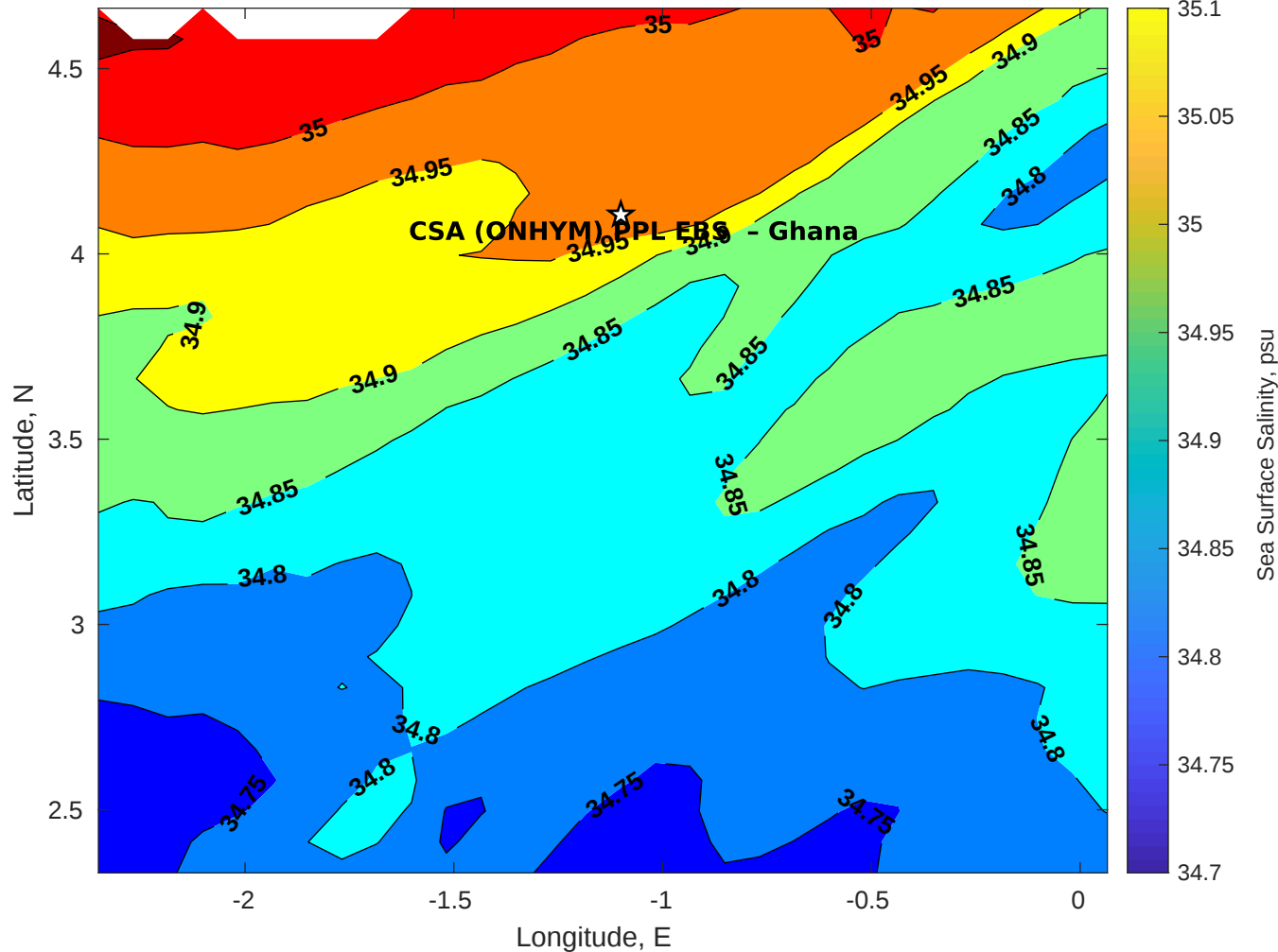
Surface Salinity for CSA (ONHYM) PPL EBS - Ghana at 21-Apr-2025 00:00:00
