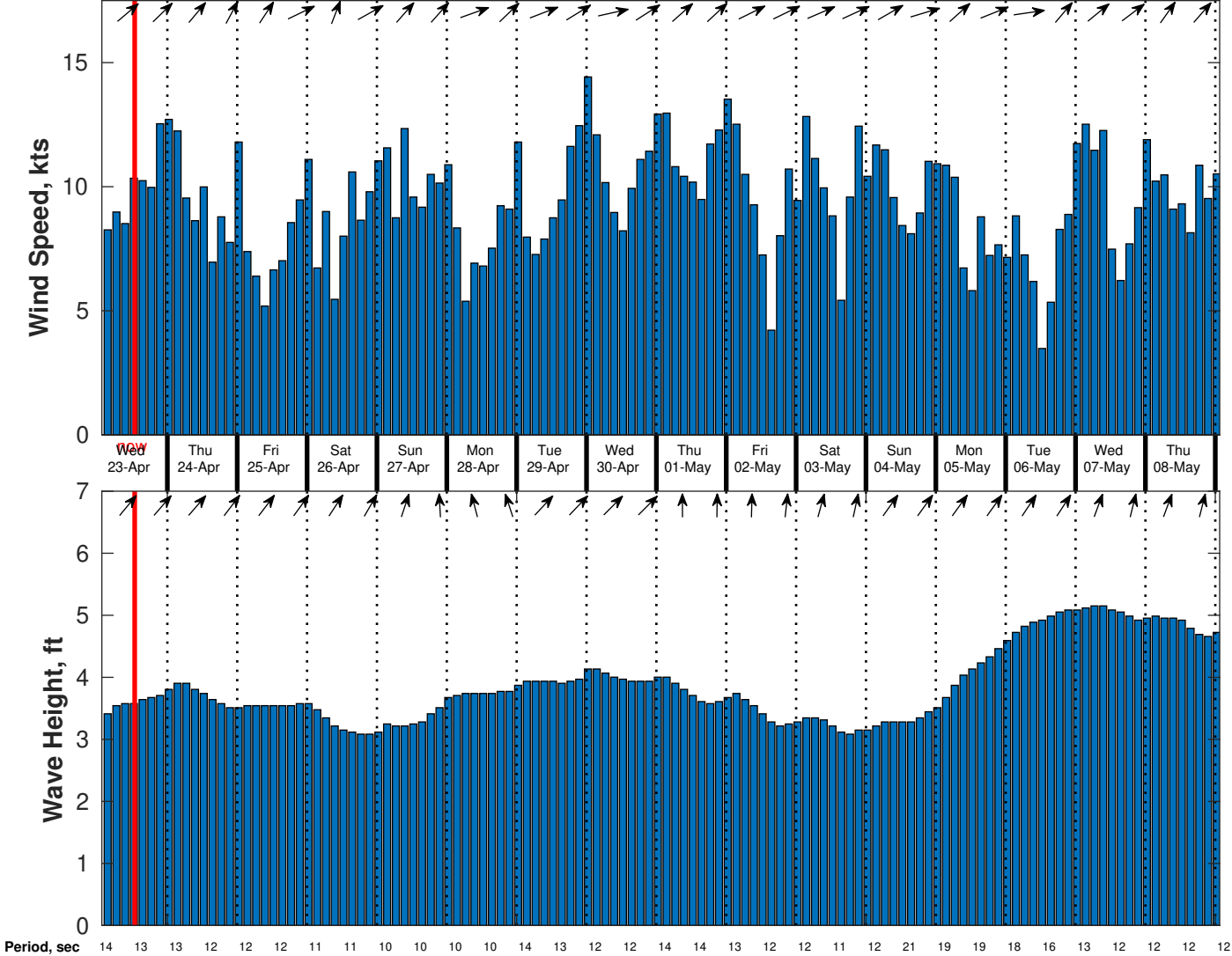
Wind & Wave Forecast for CSA (ONHYM) PPL EBS - Ghana from 22-Apr-2025 02:00:00 to 08-May-2025 02:00:00
