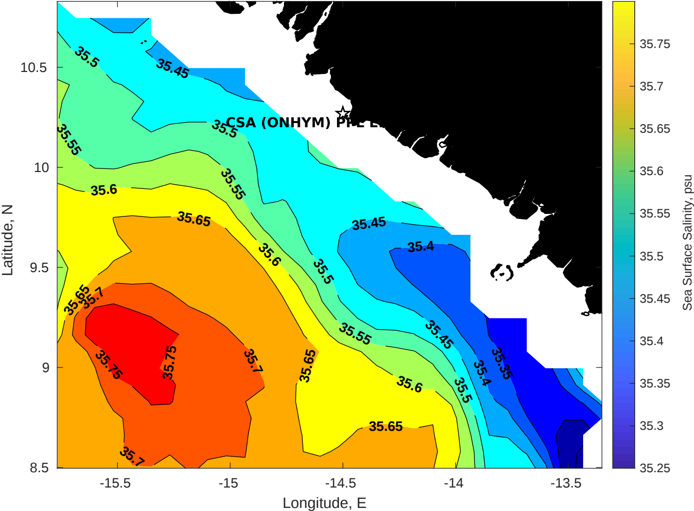
Surface Salinity for CSA (ONHYM) PPL EBS - Guinea at 21-Apr-2025 00:00:00
