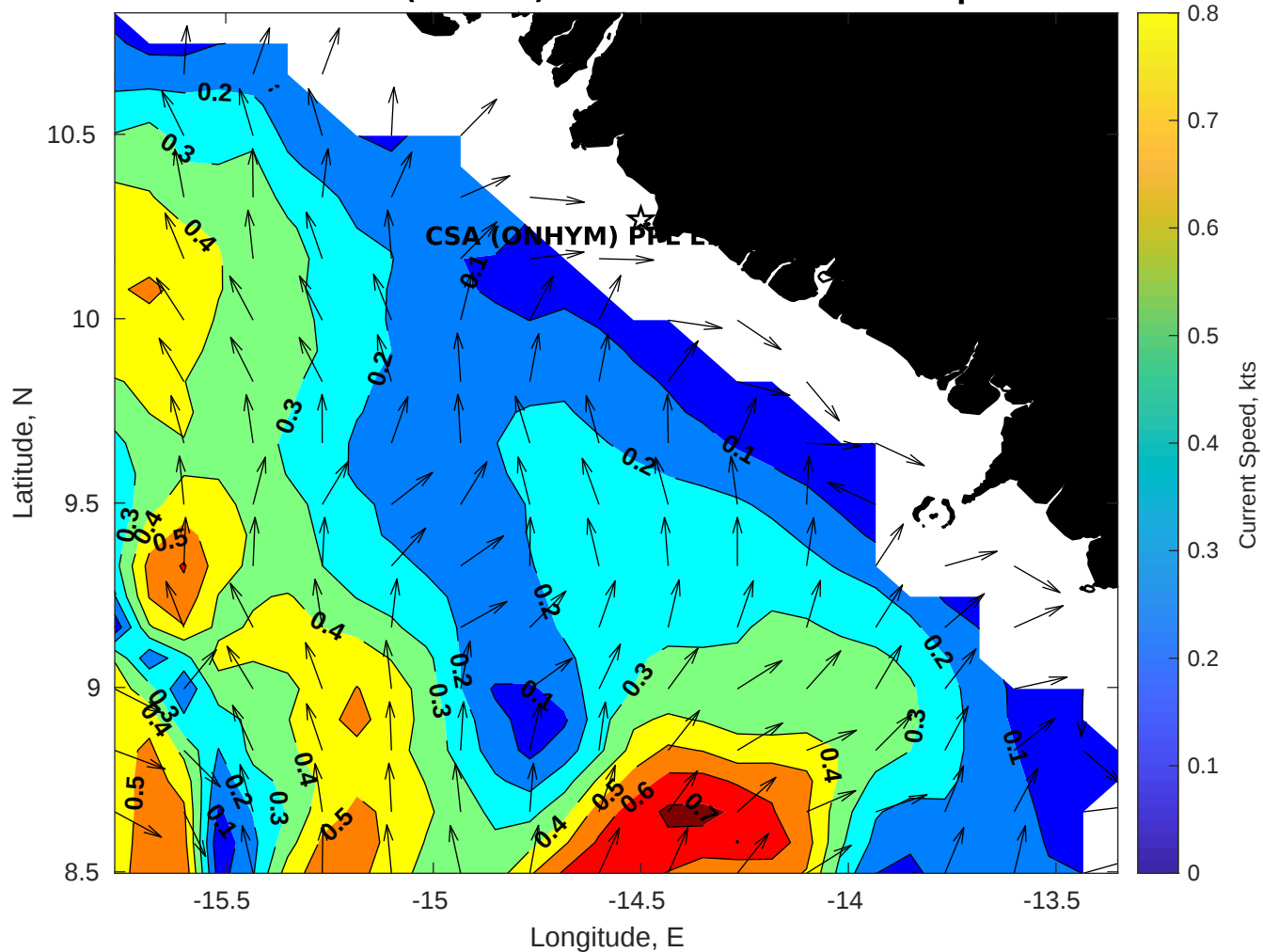
Surface Currents for CSA (ONHYM) PPL EBS - Guinea at 21-Apr-2025 00:00:00
