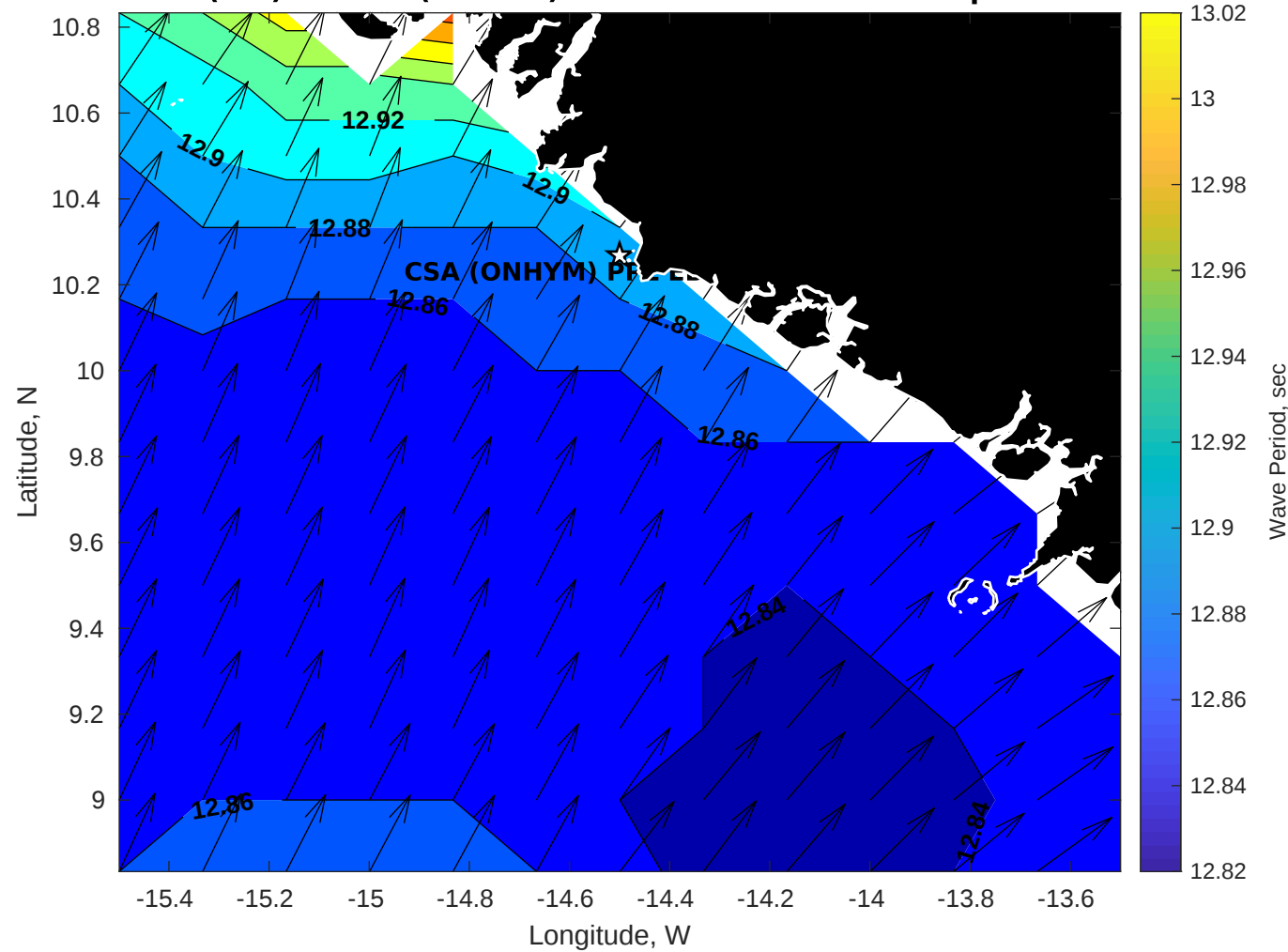
Wave Period (sec) for CSA (ONHYM) PPL EBS - Guinea at 22-Apr-2025 09:00:00
