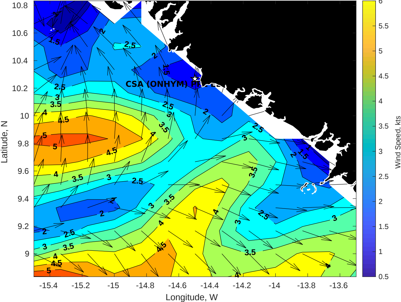
Winds (kts) for CSA (ONHYM) PPL EBS - Guinea at 22-Apr-2025 09:00:00
