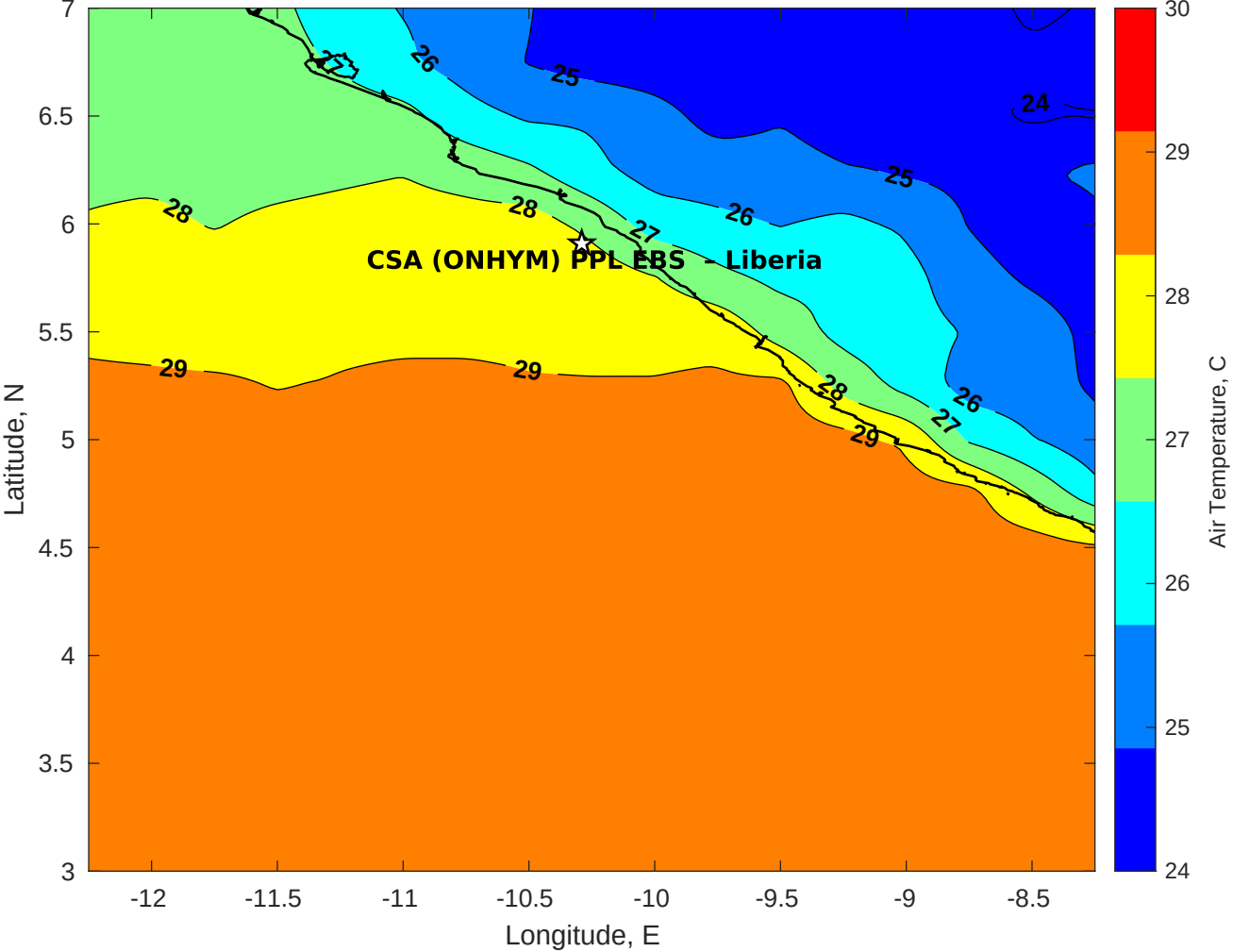
Air Temperature (C) for CSA (ONHYM) PPL EBS - Liberia at 22-Apr-2025
