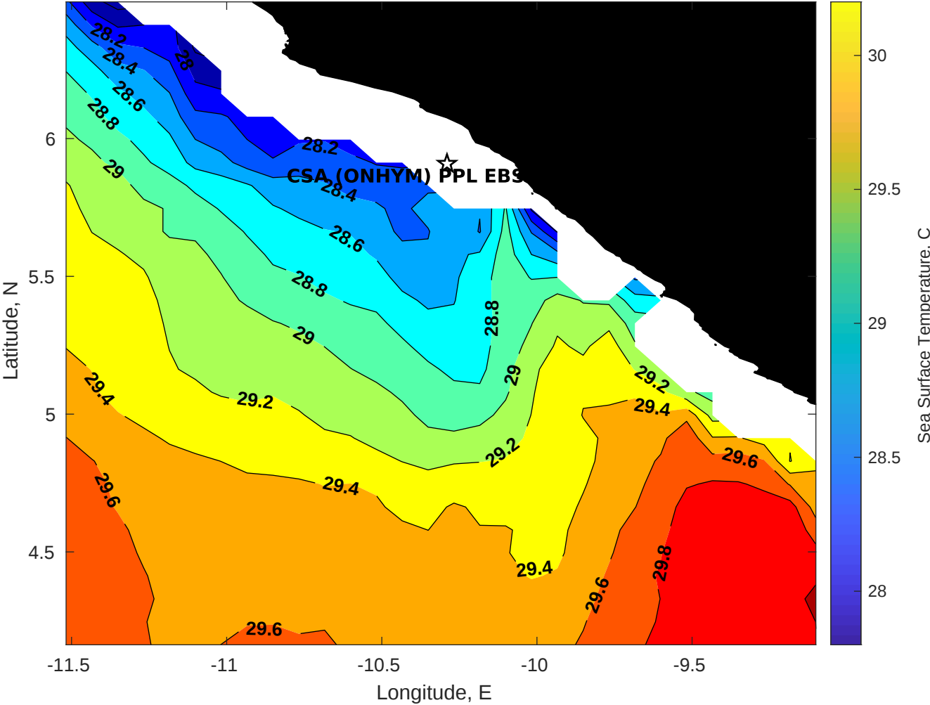
SST for CSA (ONHYM) PPL EBS - Liberia at 21-Apr-2025 00:00:00
