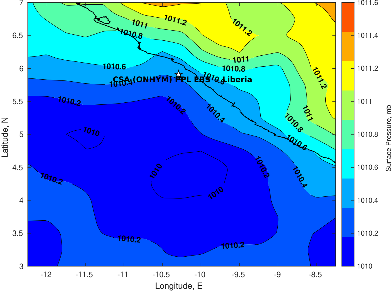
Surface Pressure (mb) for CSA (ONHYM) PPL EBS - Liberia at 23-Apr-2025 00:00:00
