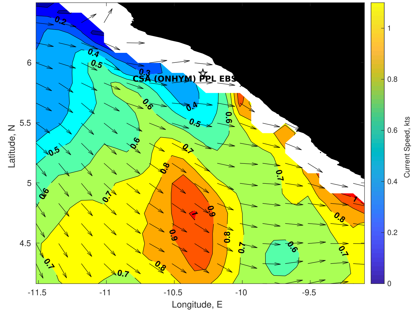
Surface Currents for CSA (ONHYM) PPL EBS - Liberia at 21-Apr-2025 00:00:00
