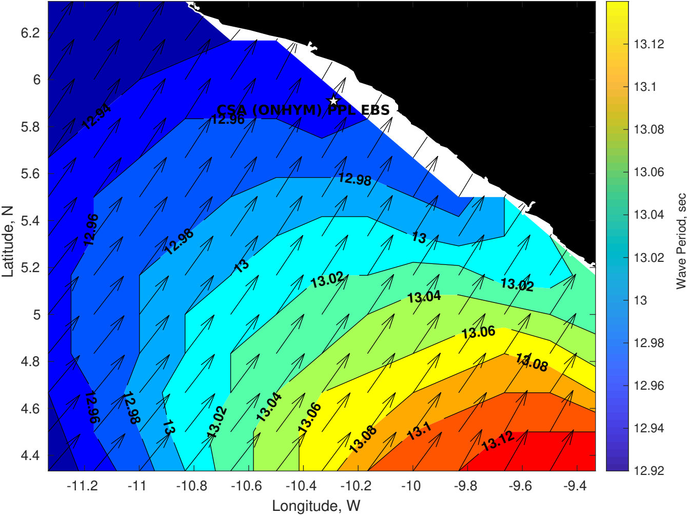
Wave Period (sec) for CSA (ONHYM) PPL EBS - Liberia at 22-Apr-2025 09:00:00
