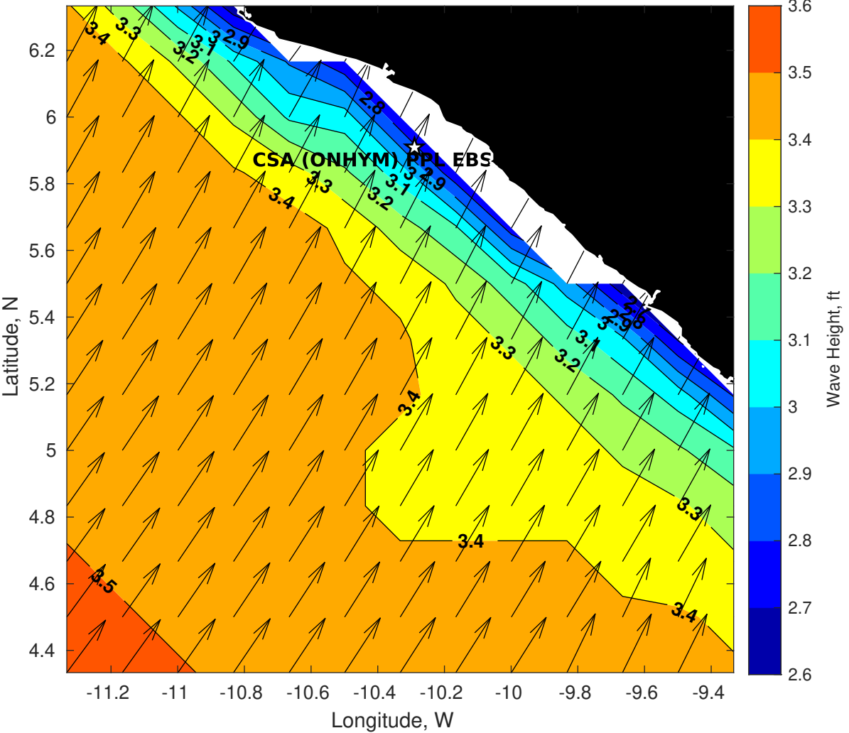
Wave Height (ft) for CSA (ONHYM) PPL EBS - Liberia at 22-Apr-2025 09:00:00
