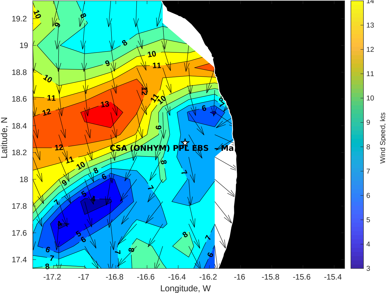
Winds (kts) for CSA (ONHYM) PPL EBS - Mauritania at 22-Apr-2025 09:00:00
