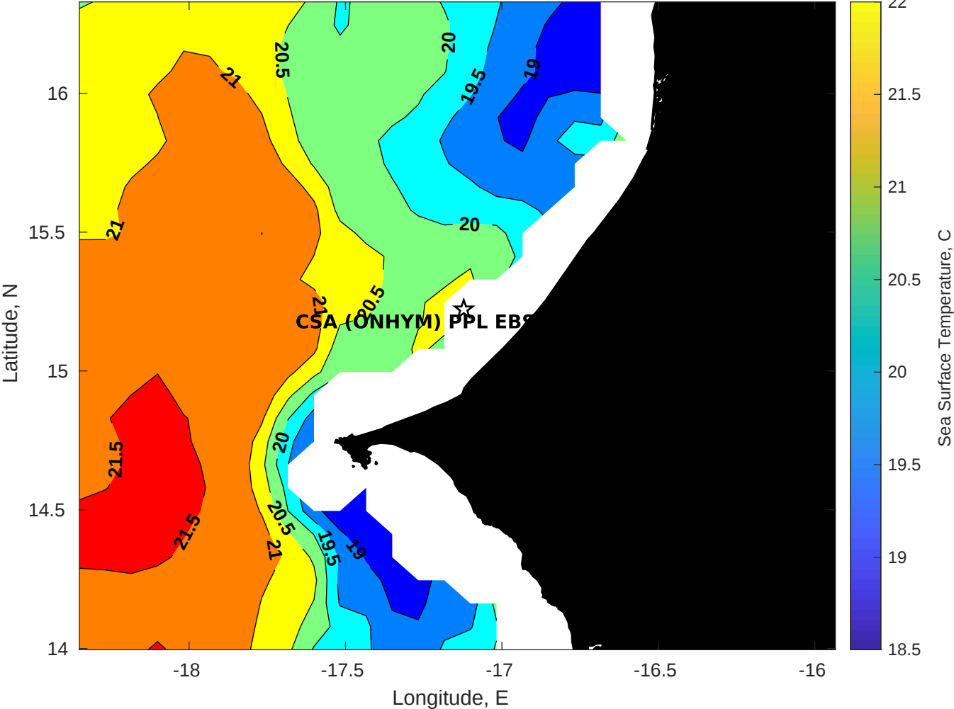
SST for CSA (ONHYM) PPL EBS - Senegal at 21-Apr-2025 00:00:00
