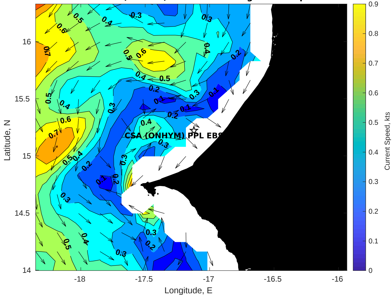
Surface Currents for CSA (ONHYM) PPL EBS - Senegal at 21-Apr-2025 00:00:00
