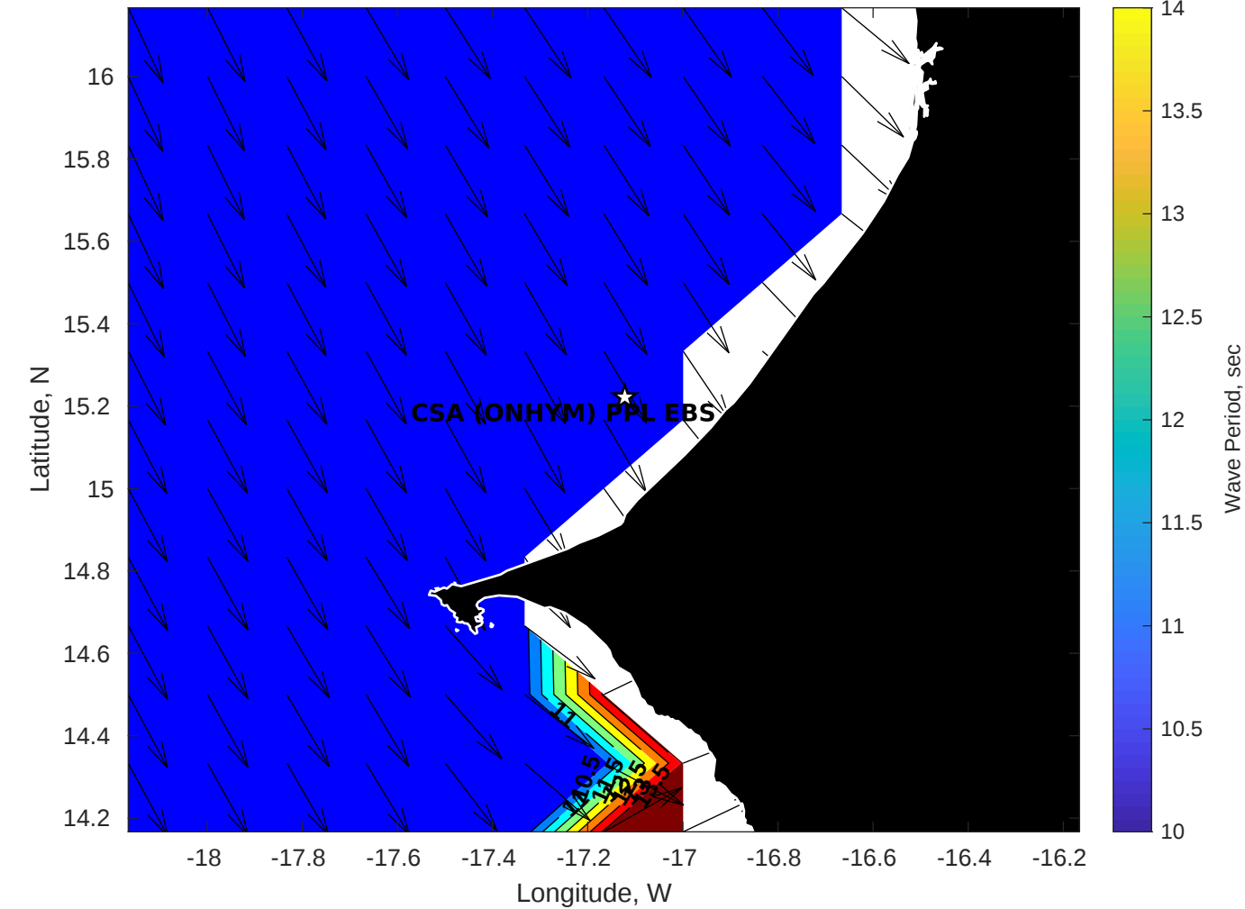
Wave Period (sec) for CSA (ONHYM) PPL EBS - Senegal at 22-Apr-2025 09:00:00
