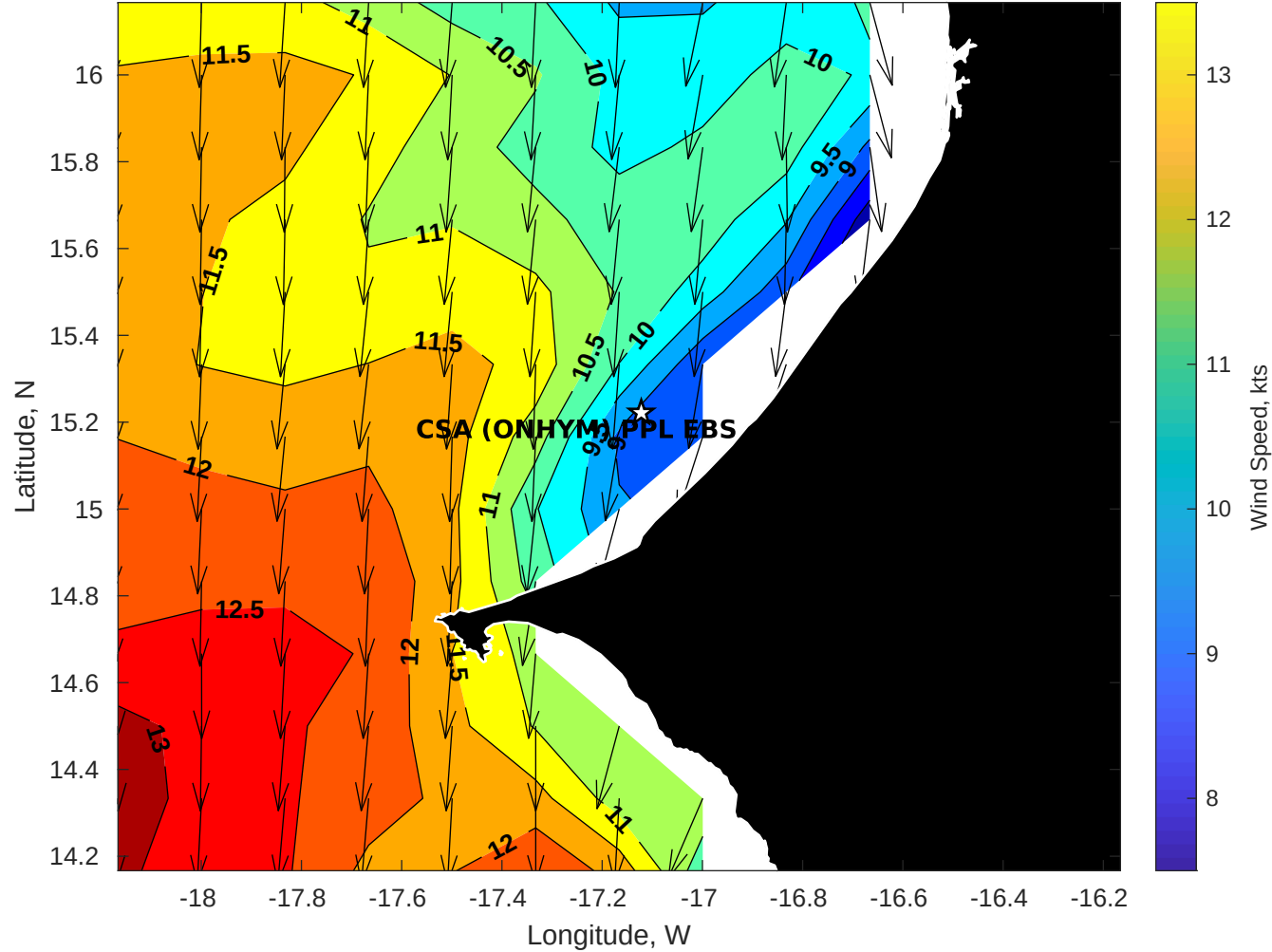
Winds (kts) for CSA (ONHYM) PPL EBS - Senegal at 22-Apr-2025 09:00:00
