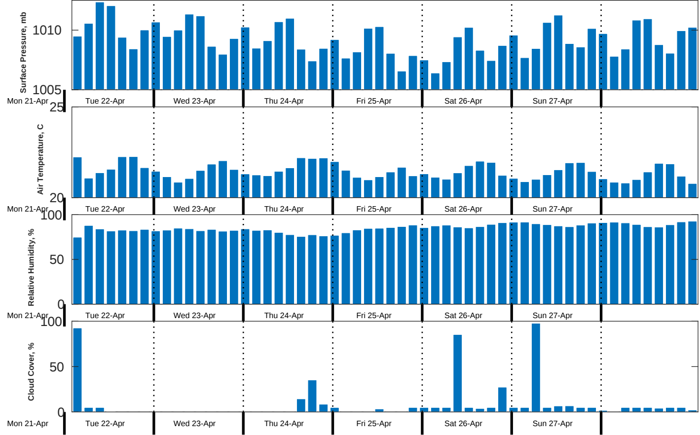
Met Forecast for CSA (ONHYM) PPL EBS - Senegal from 22-Apr-2025 00:00:00 to 29-Apr-2025 00:00:00
