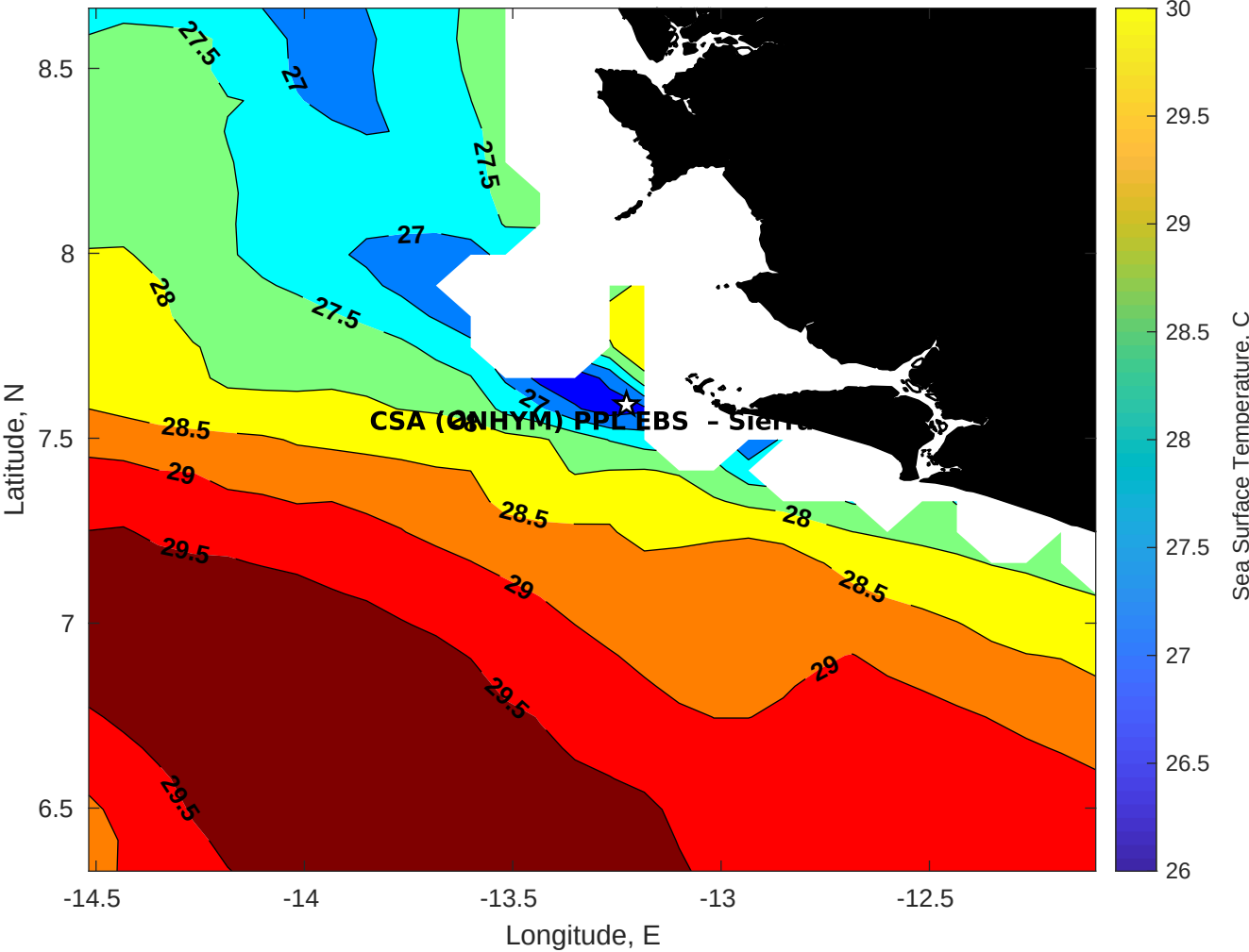
SST for CSA (ONHYM) PPL EBS - Sierra Leone at 21-Apr-2025 00:00:00
