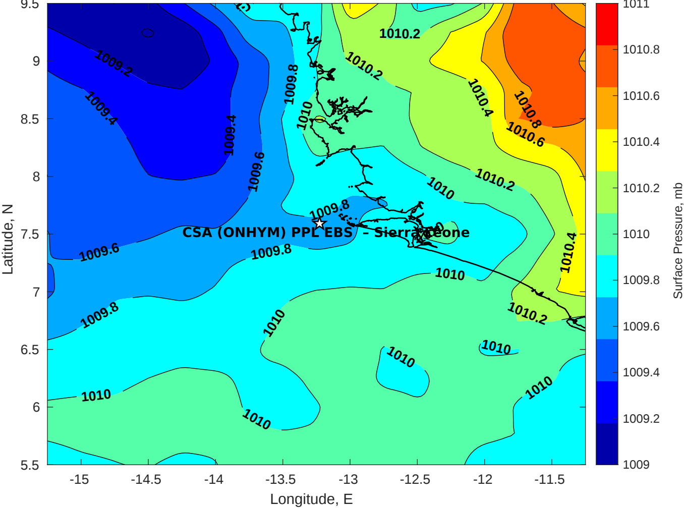
Surface Pressure (mb) for CSA (ONHYM) PPL EBS - Sierra Leone at 22-Apr-2025 00:00:00
