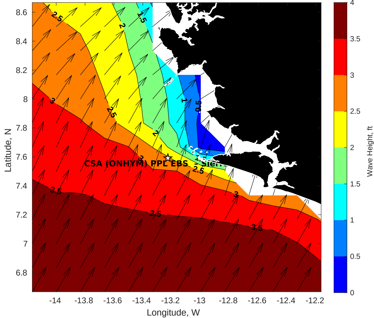
Wave Height (ft) for CSA (ONHYM) PPL EBS - Sierra Leone at 22-Apr-2025 09:00:00
