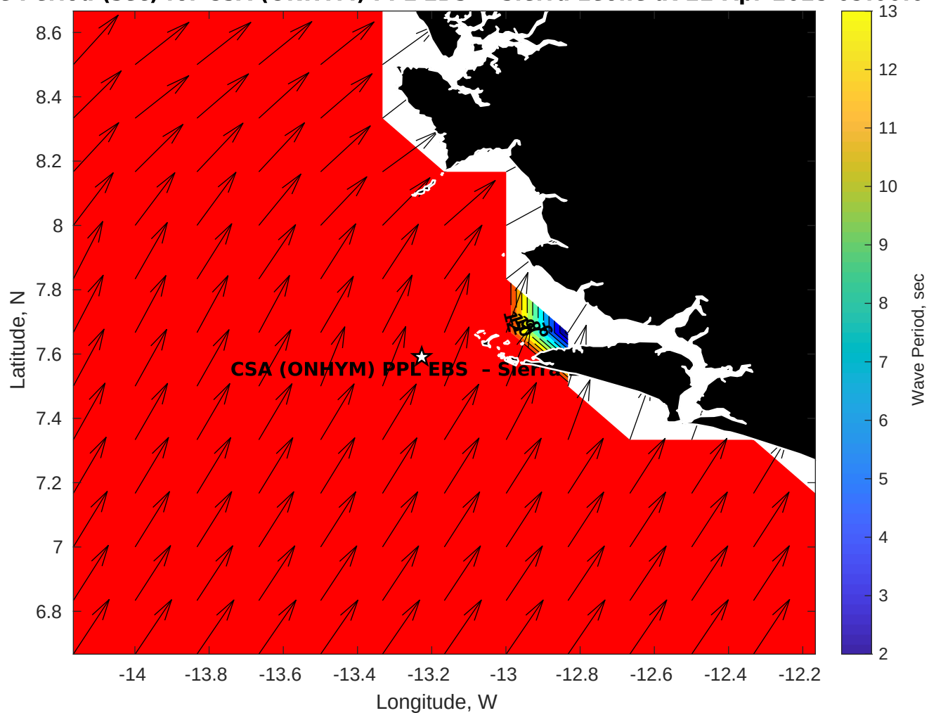
Wave Period (sec) for CSA (ONHYM) PPL EBS - Sierra Leone at 22-Apr-2025 09:00:00
