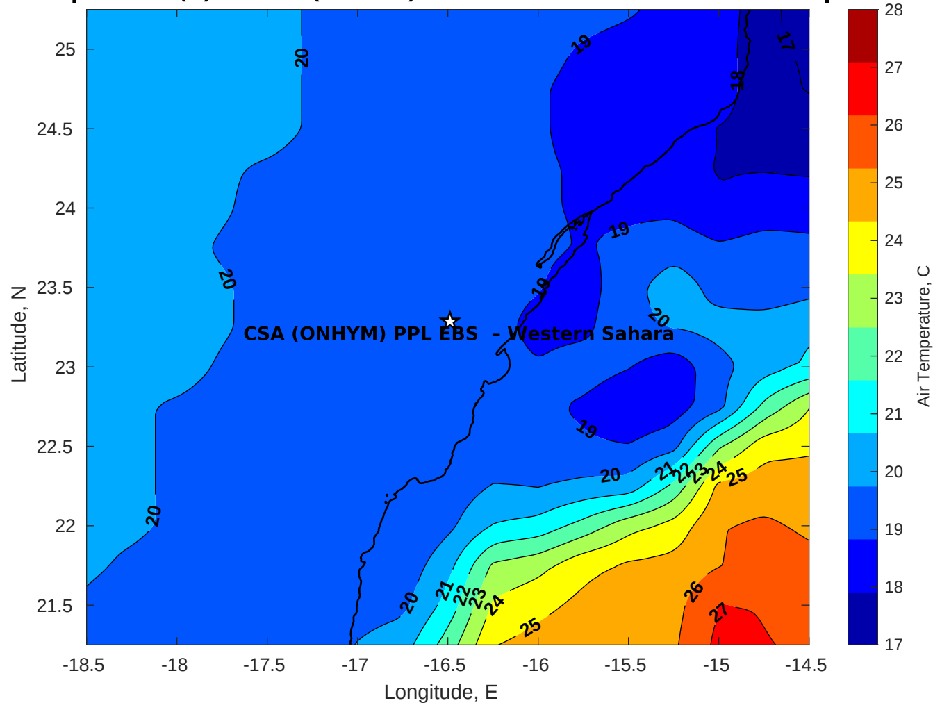
Air Temperature (C) for CSA (ONHYM) PPL EBS - Western Sahara at 22-Apr-2025
