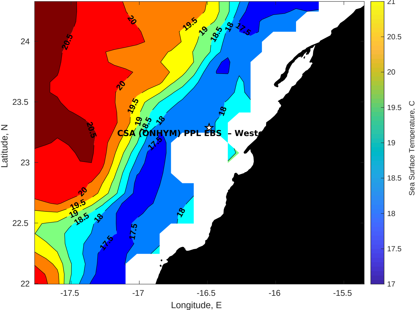
SST for CSA (ONHYM) PPL EBS - Western Sahara at 21-Apr-2025 00:00:00
