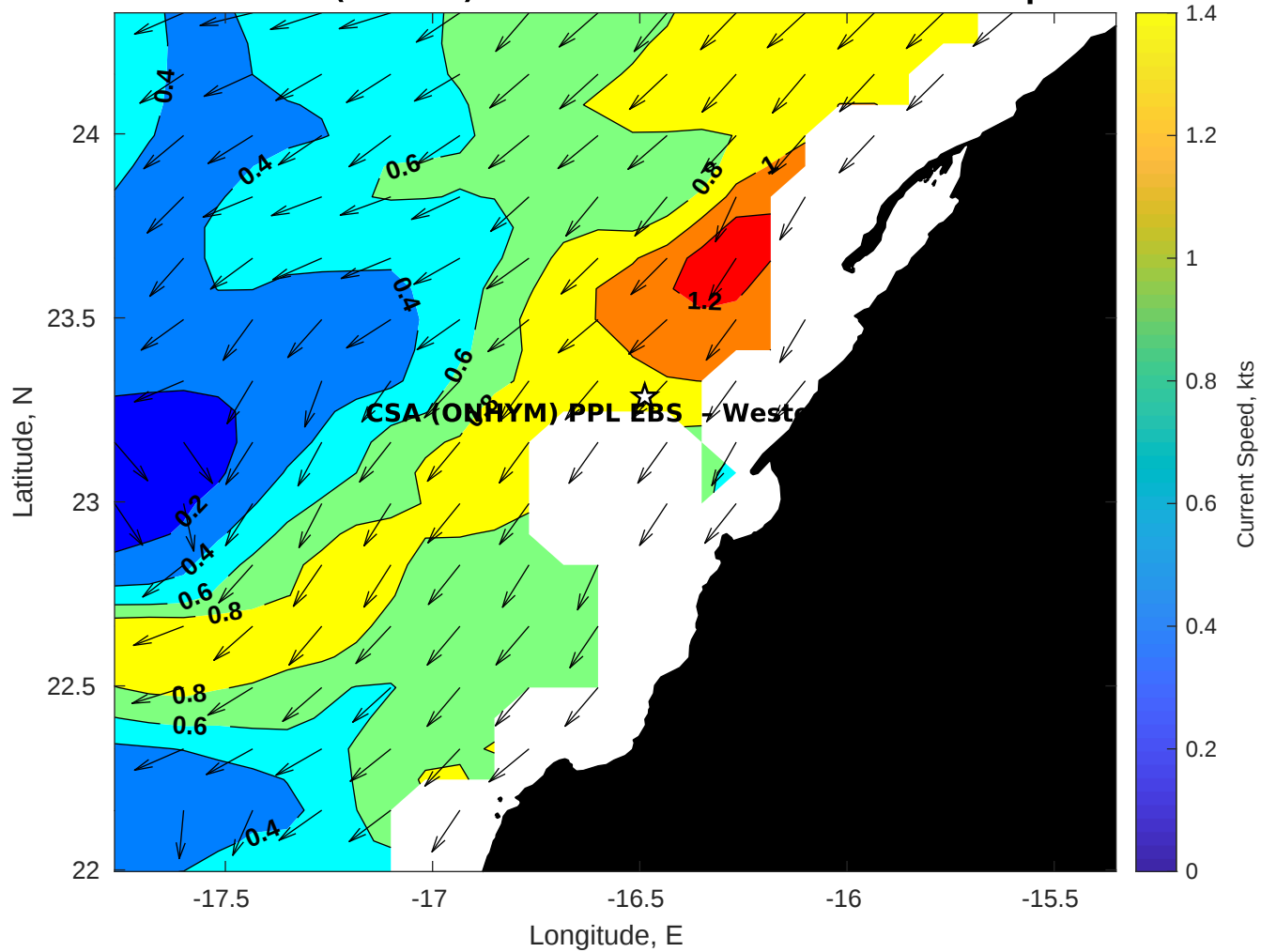
Surface Currents for CSA (ONHYM) PPL EBS - Western Sahara at 21-Apr-2025 00:00:00
