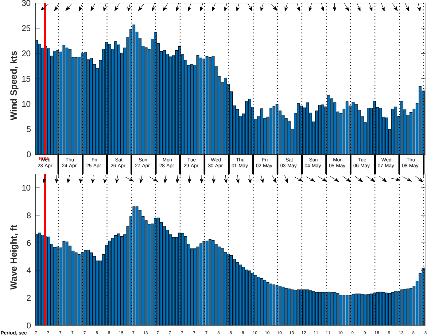
Wind & Wave Forecast for CSA (ONHYM) PPL EBS - Western Sahara from 22-Apr-2025 01:00:00 to 08-May-2025 01:00:00
