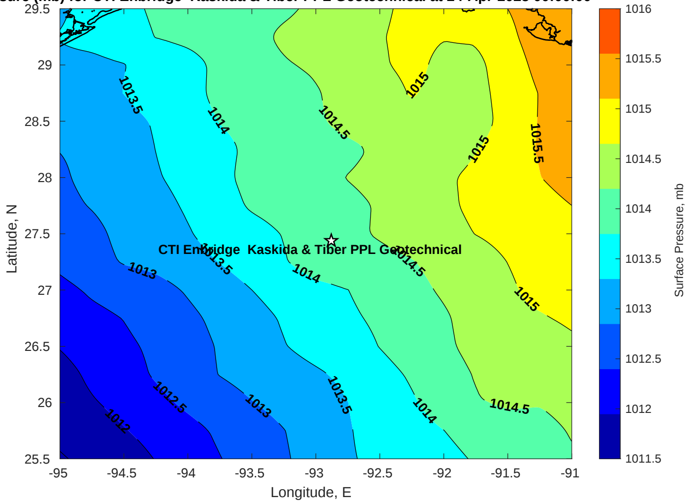
Surface Pressure (mb) for CTI Enbridge Kaskida & Tiber PPL Geotechnical at 24-Apr-2025 00:00:00
