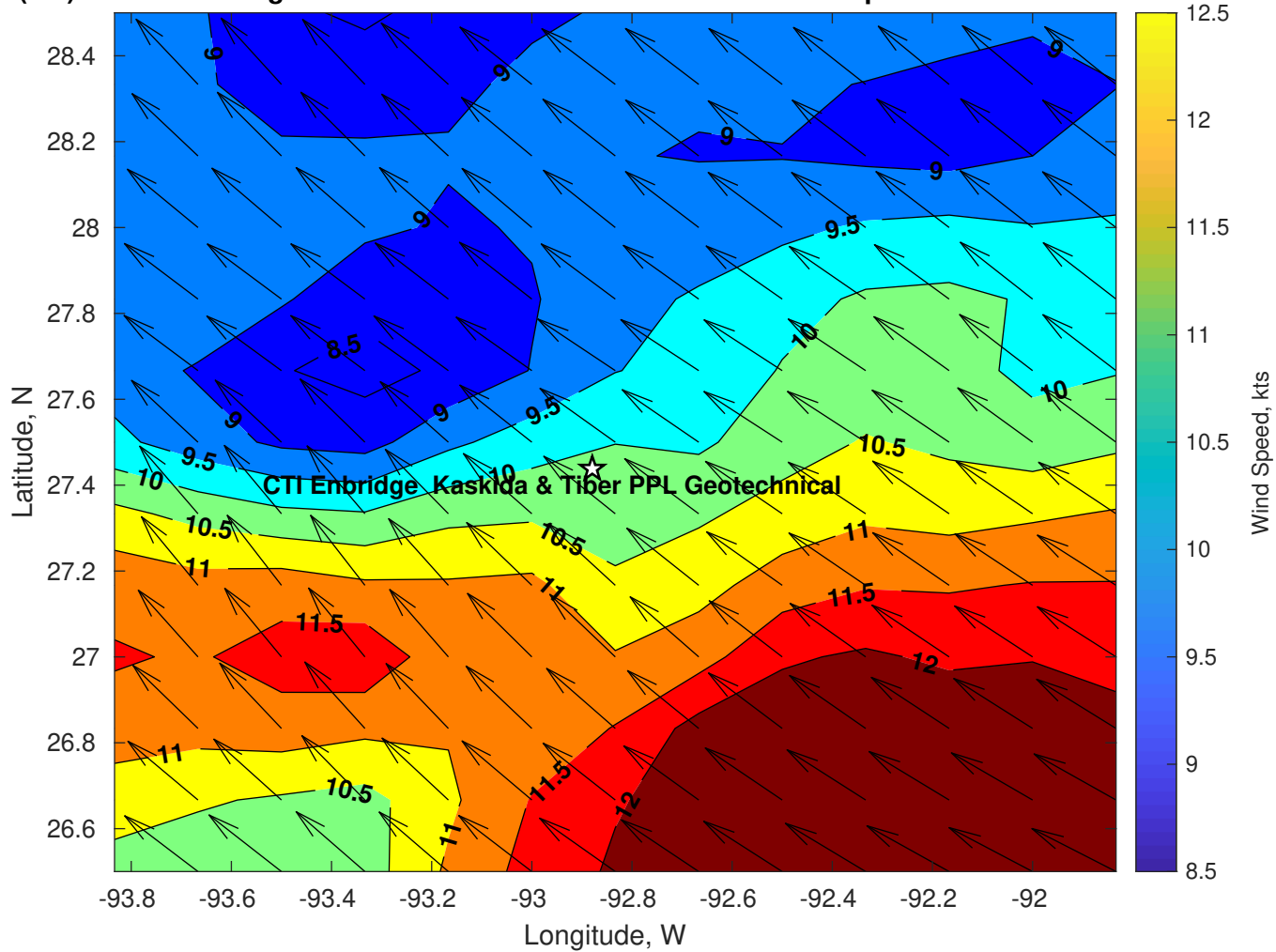
Winds (kts) for CTI Enbridge Kaskida & Tiber PPL Geotechnical at 22-Apr-2025 09:00:00
