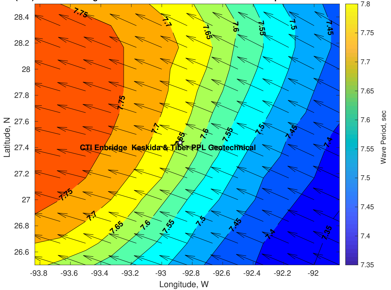
Wave Period (sec) for CTI Enbridge Kaskida & Tiber PPL Geotechnical at 22-Apr-2025 09:00:00
