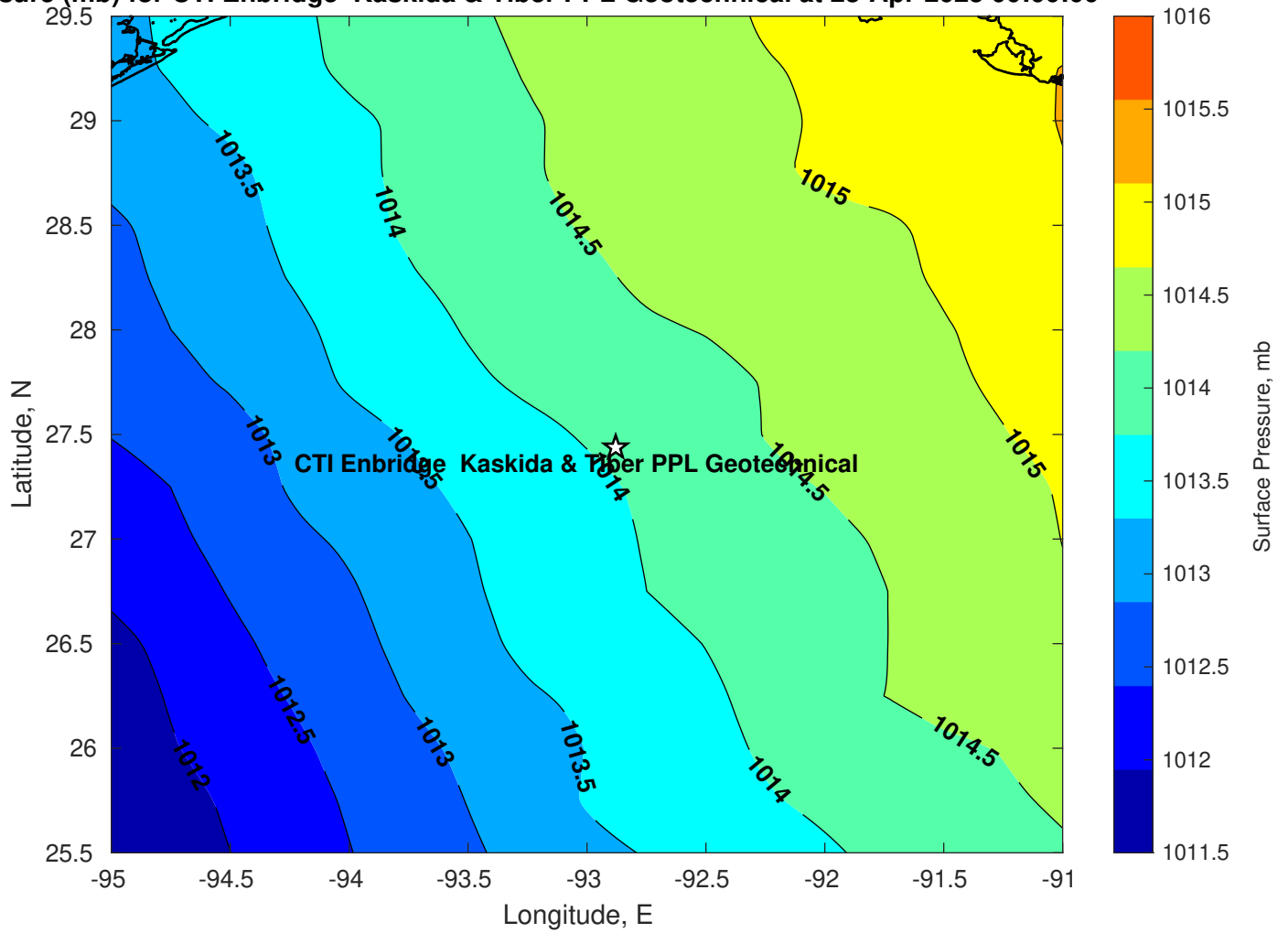
Surface Pressure (mb) for CTI Enbridge Kaskida & Tiber PPL Geotechnical at 23-Apr-2025 00:00:00
