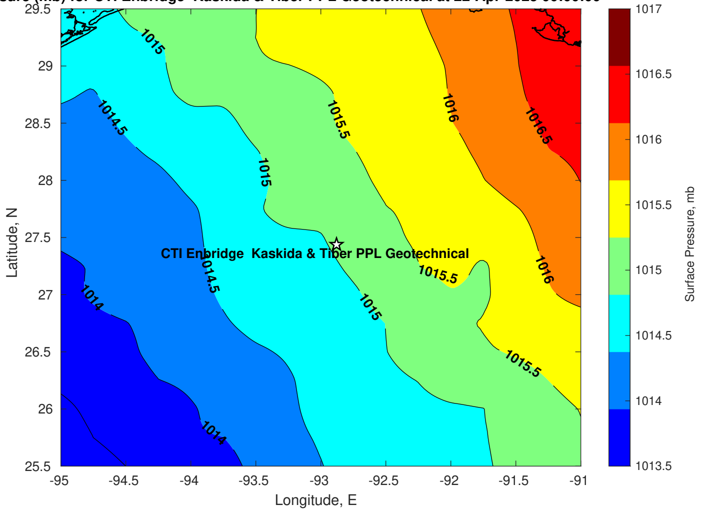
Surface Pressure (mb) for CTI Enbridge Kaskida & Tiber PPL Geotechnical at 22-Apr-2025 00:00:00
