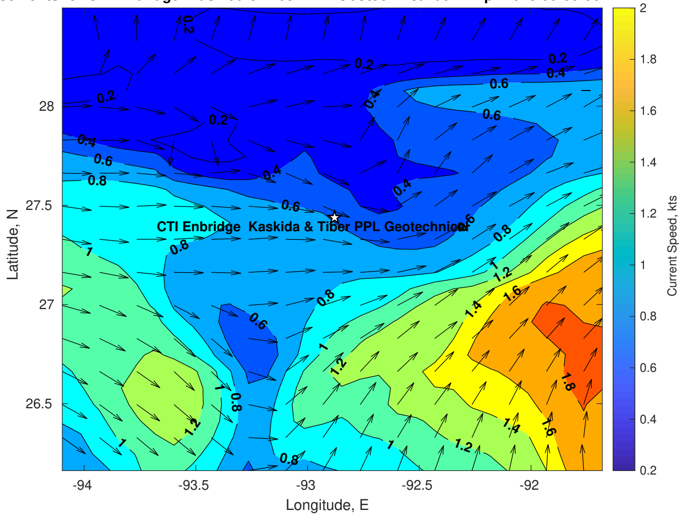
Surface Currents for CTI Enbridge Kaskida & Tiber PPL Geotechnical at 21-Apr-2025 00:00:00
