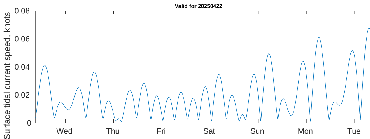
Tidal Currents and Heights for CTI Enbridge Kaskida & Tiber PPL Geotechnical at 20250422
