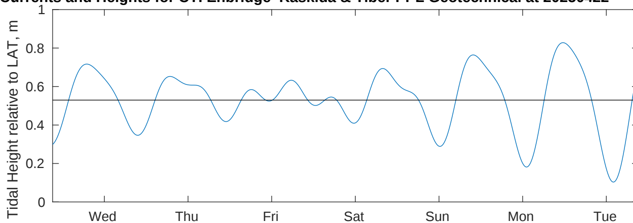
Tidal Currents and Heights for CTI Enbridge Kaskida & Tiber PPL Geotechnical at 20250422
