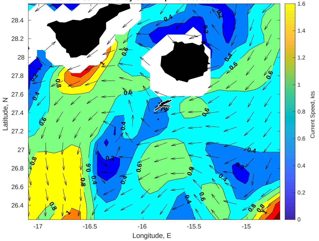
Surface Currents for Gyre at 21-Apr-2025 00:00:00
