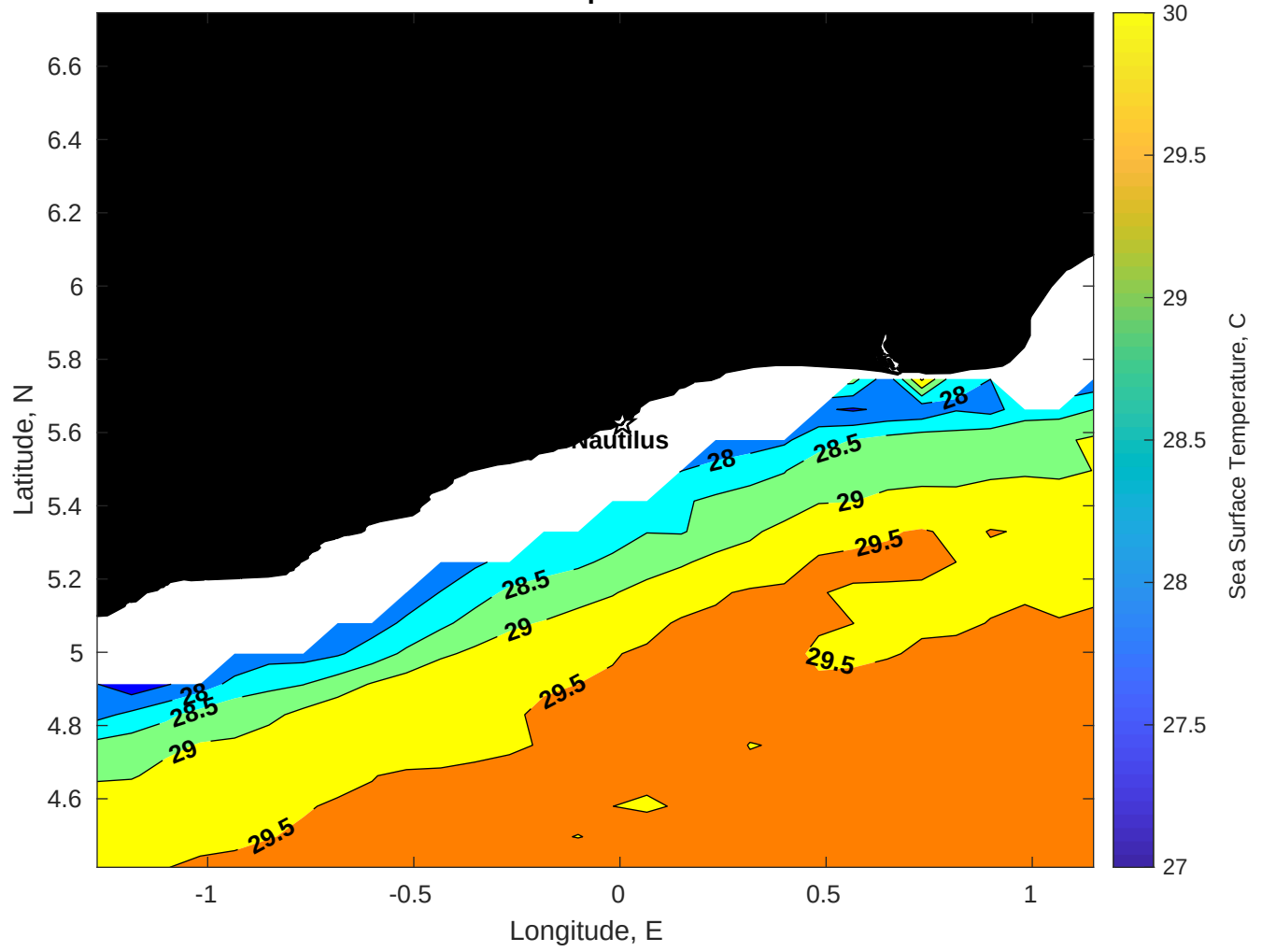
SST for Nautilus at 21-Apr-2025 00:00:00
