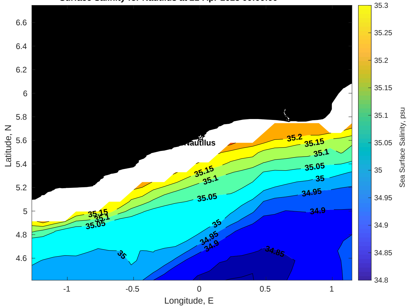
Surface Salinity for Nautilus at 21-Apr-2025 00:00:00
