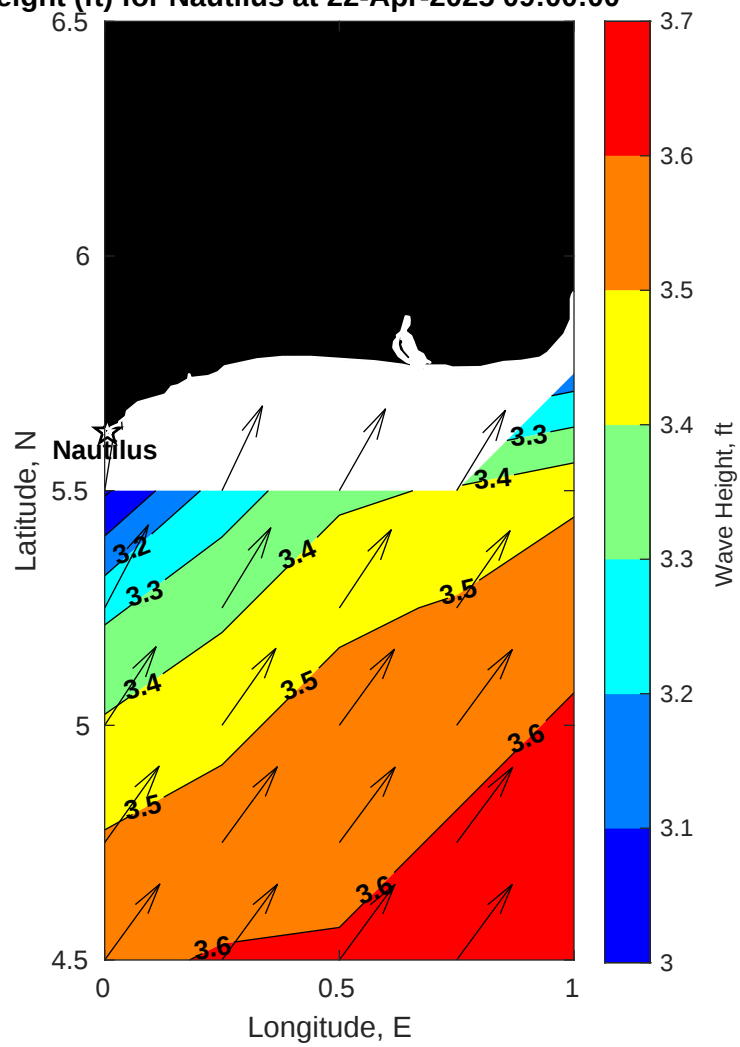
Wave Height (ft) for Nautilus at 22-Apr-2025 09:00:00
