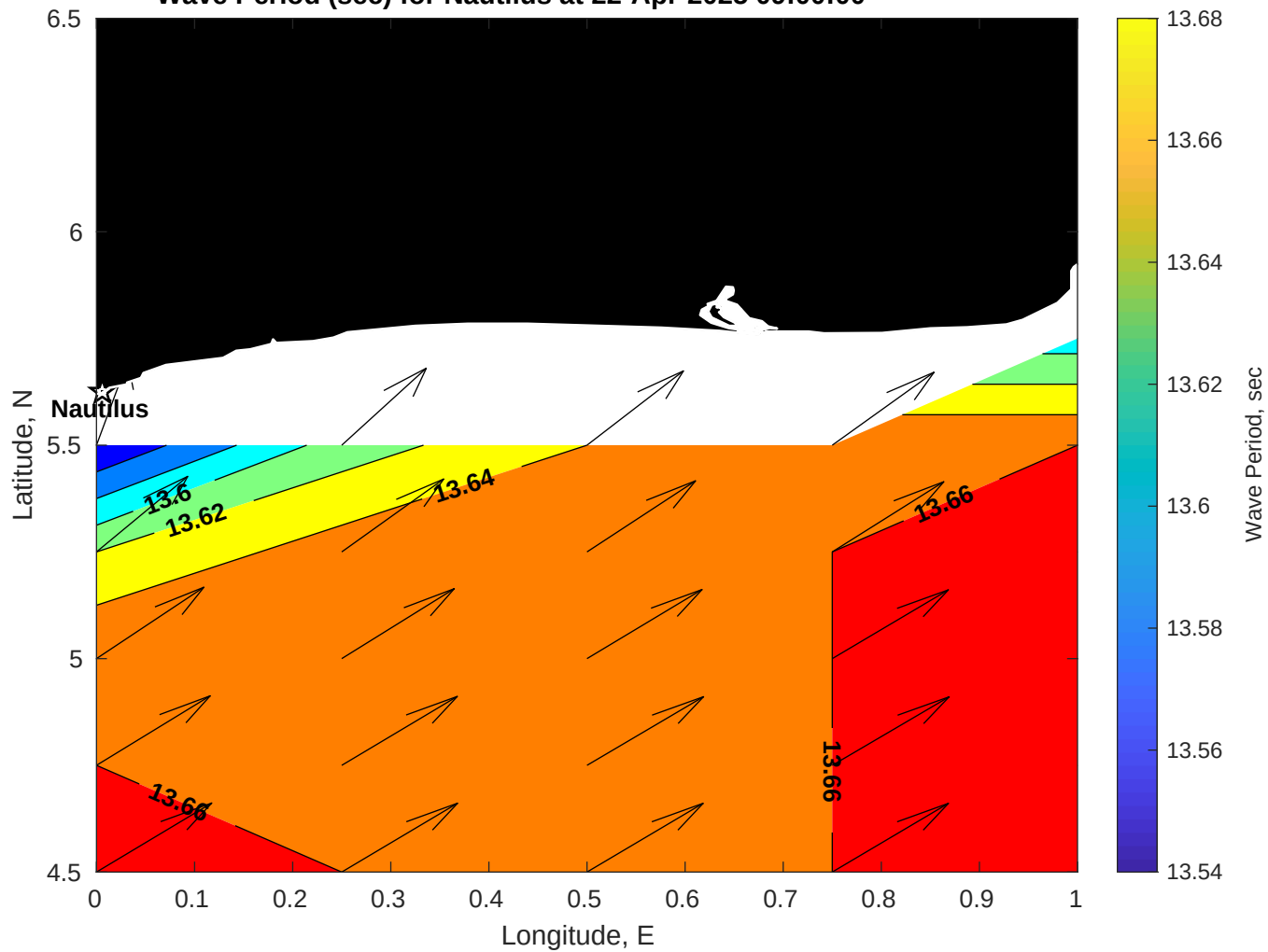
Wave Period (sec) for Nautilus at 22-Apr-2025 09:00:00
